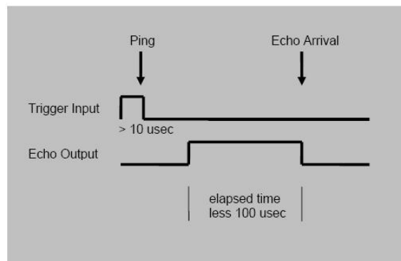
Figure 2 - Devantech SRF04 Signals
