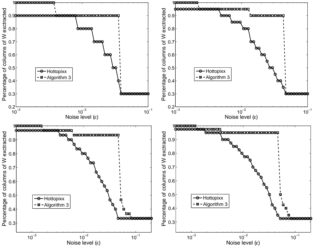
Figure 1: Comparison of Hottopixx and Algorithm 3 on the near-separable matrices from Theorem 7 with duplicates of the columns of W . From left to right, top to bottom: r = 10, 20, 30, 40 .
