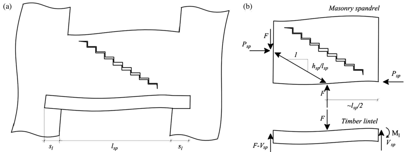
Figure 11-3. Shear Mechanism of URM Spandrels with Lintels
