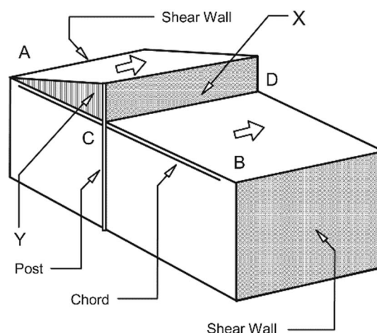
Figure A-31. Roof Chord Continuity
