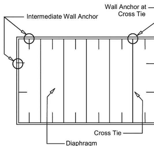
Figure A-30. Cross Ties
