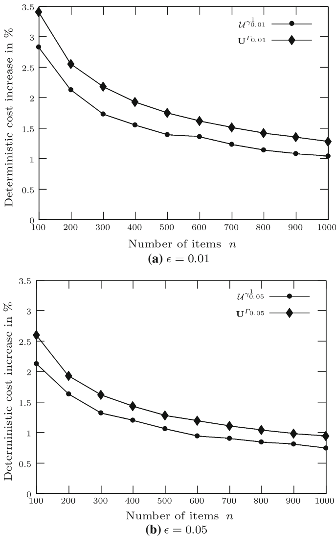
Fig. 3 Cost of protecting the solution for the knapsack problem
