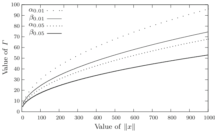
Fig. 1 Comparison of the two bounds
