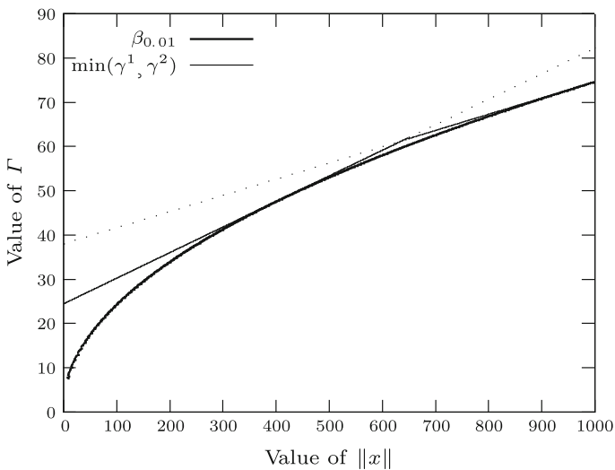
(b) Two piece-wise linear functions
