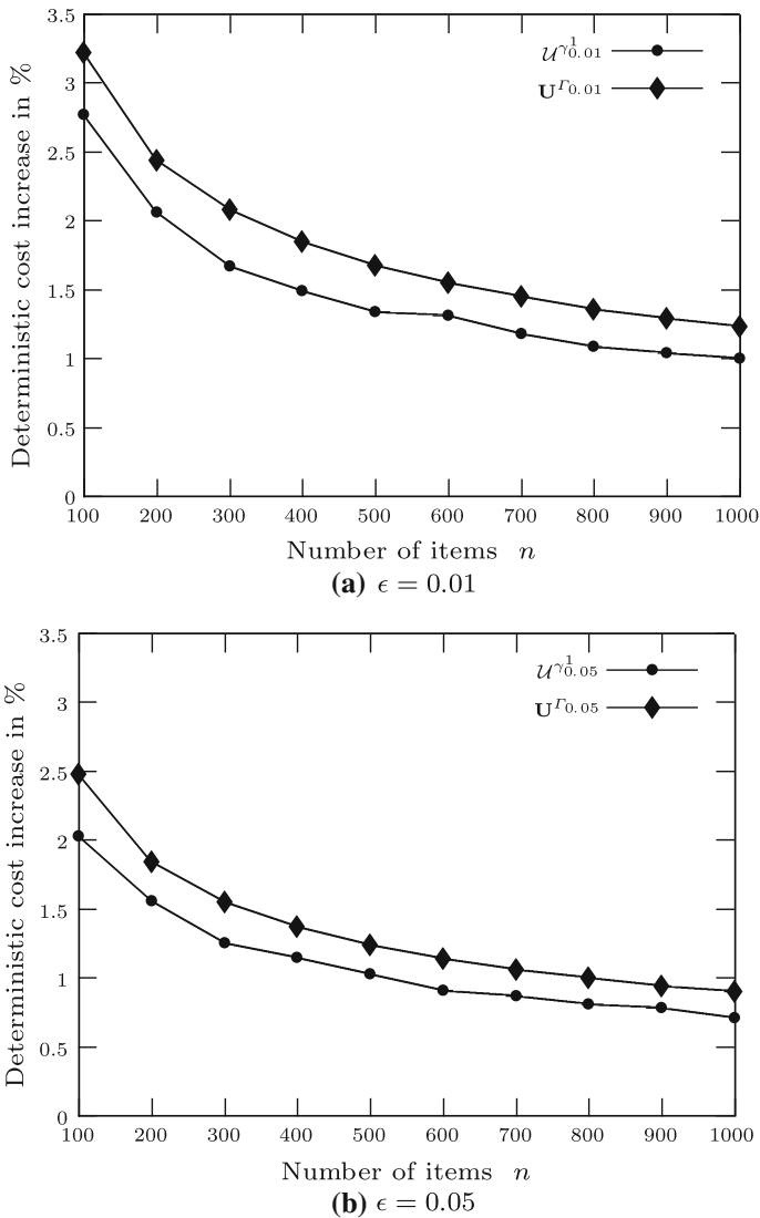
Fig. 4 Cost of protecting the solution for the fractional knapsack problem
