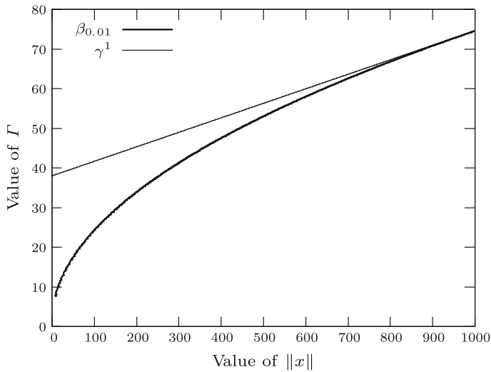
(a) One piece-wise linear function
