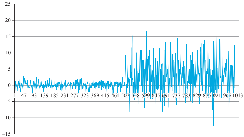
Figure 10.1 Sample time series plot illustrating a regime shift
