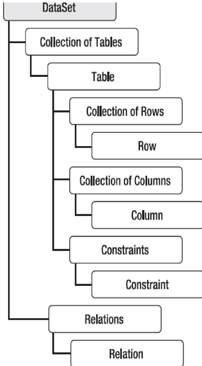
Figure 13-1. Dataset architecture
