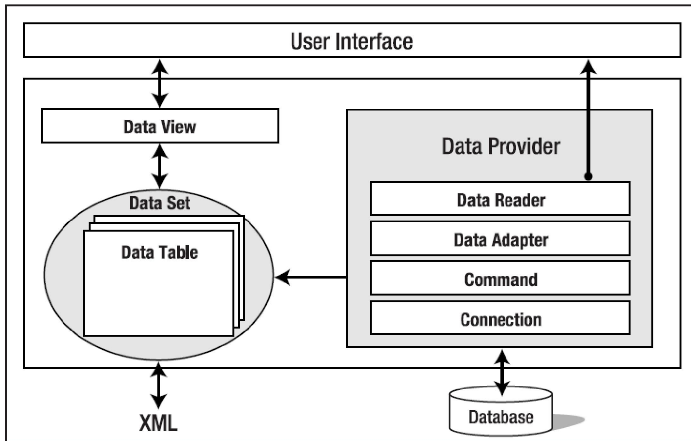
Figure 9-1. ADO.NET architecture
