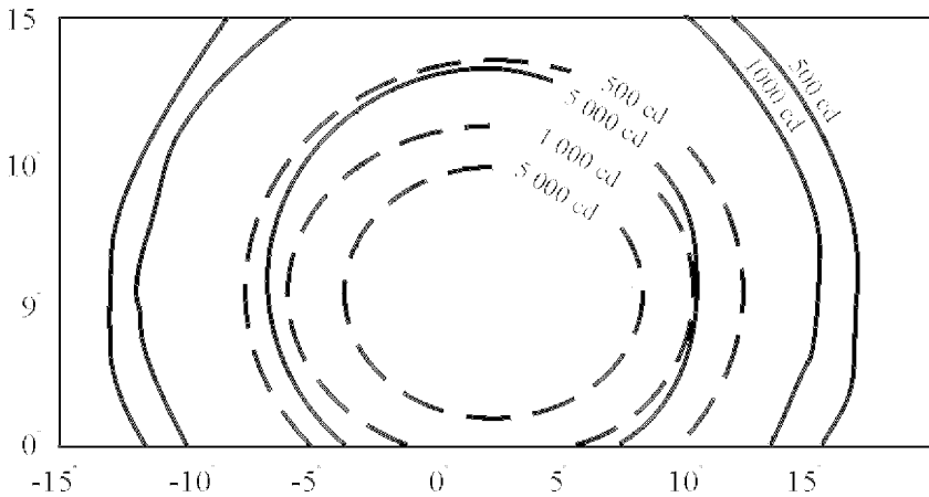
Figure 15-7 Isocandela diagram EL-AT [cd], threshold light (green light)
