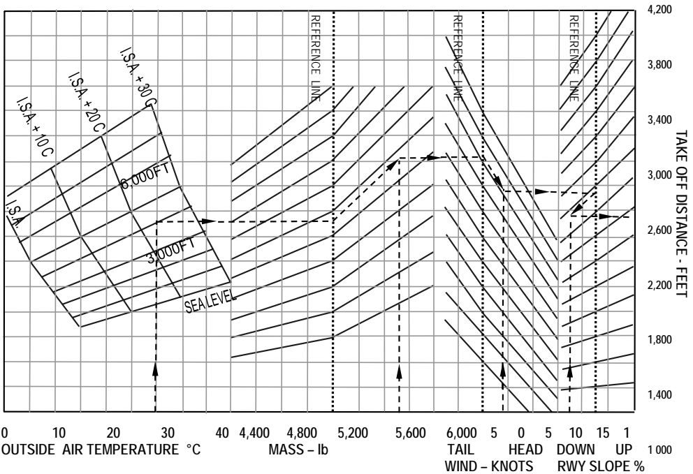
Figure 4-2 Single engine piston aeroplane take-off distance
