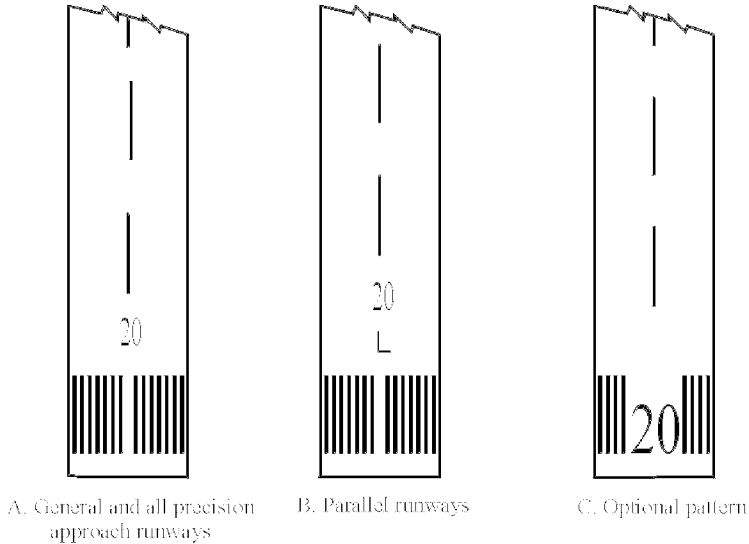
Figure 15-2a Runway designation, centre line and threshold markings (Source: Annex 14, Aerodromes, Volume I, Aerodrome Design and Operations)
