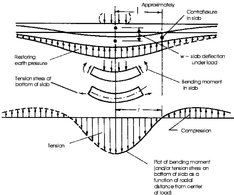
Figure 8-10 Physical meaning of Westergaards 'radius of relative stiffness' P (Source: Aerodrome Design Manual, Part 3 Pavements, ICAO Doc 9157-AN/901 )
