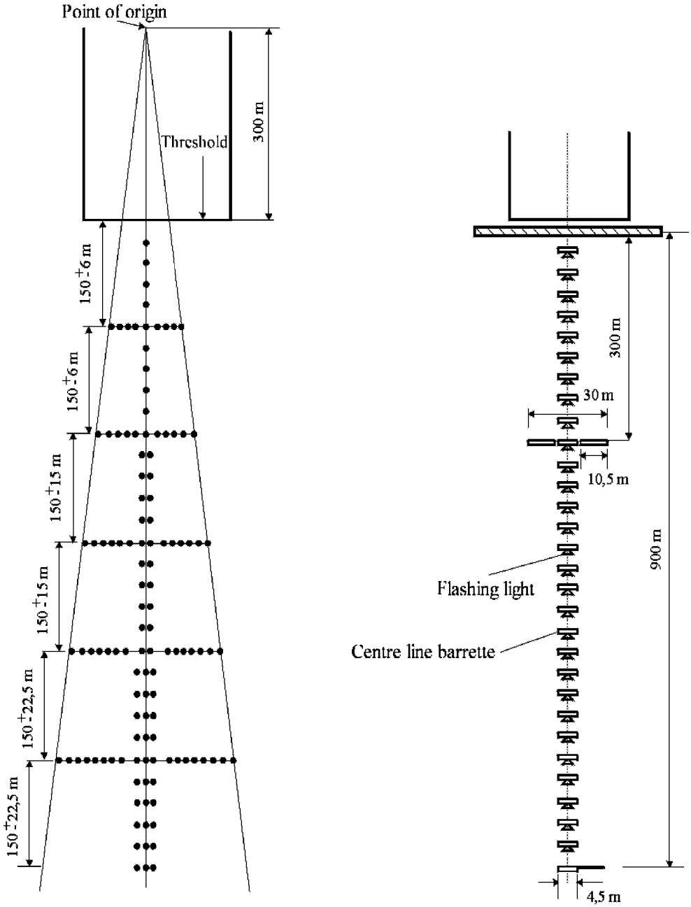
Figure 15-10 Precision approach Category I lighting systems
