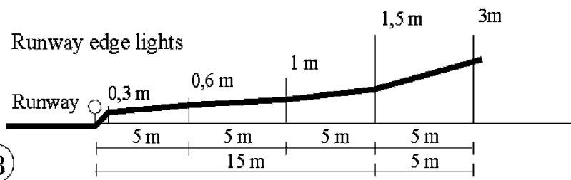
Figure 18-1 Maximum height of snowbanks
