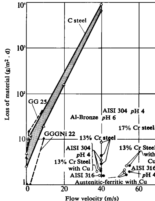
Figure 4. Erosion/Corrosion Test.
