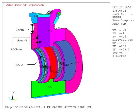
Figure 29. Area of Interest for Opening Compensation of Suction Nozzle.
