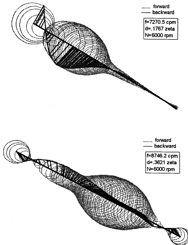
Figure 44. Damped Eigenvalue Mode Shape Plot, Worn-Condition.
