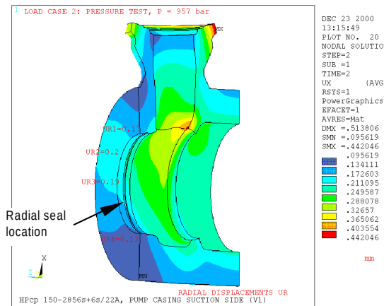
Figure 31. Radial Displacements of Barrel End at Test Conditions.
