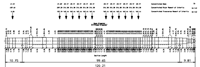
Figure 34. Rotor Model.
