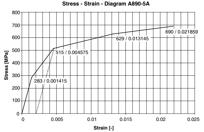
Figure 23. Stress Strain Relation of Suction Casing Material with Yield Stress of 515 MPa and Tensile Strength of 690 MPa.
