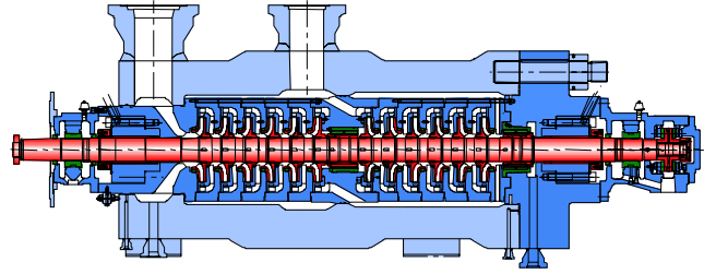
Figure 8. Prototype Pump Design.
