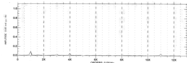
Figure 48. Frequency Spectrum at 6000 RPM and 332 M 3 /H (1462 GPM) Rated Flow, Worn-Condition.
