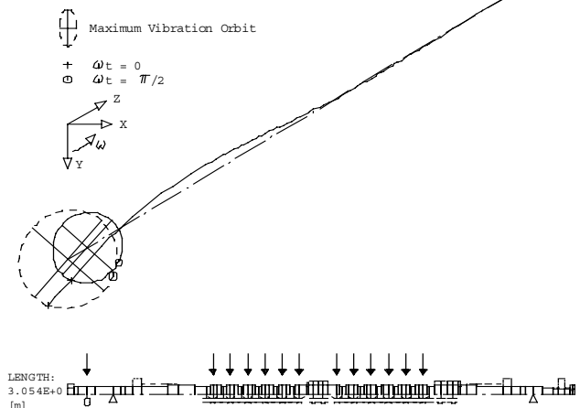
Figure 42. Coupling Sensitivity at 6000 RPM, Worn-Condition.
