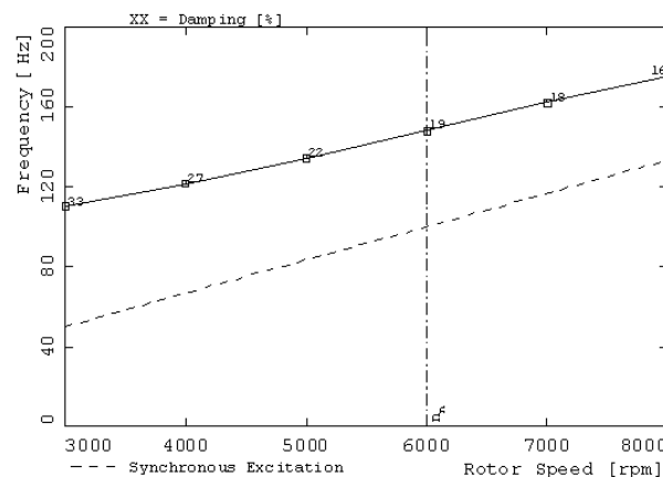
Figure 36. Campbell Diagram, New-Condition.
