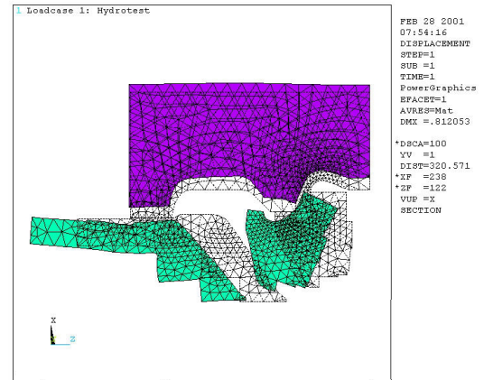
Figure 24. Distortion of Suction Casing and Barrel at Load Case Hydrotest.
