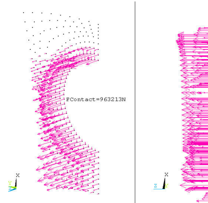
Figure 18. Nodal Contact Forces at Cover Flange for Load Case Hydrotest.
