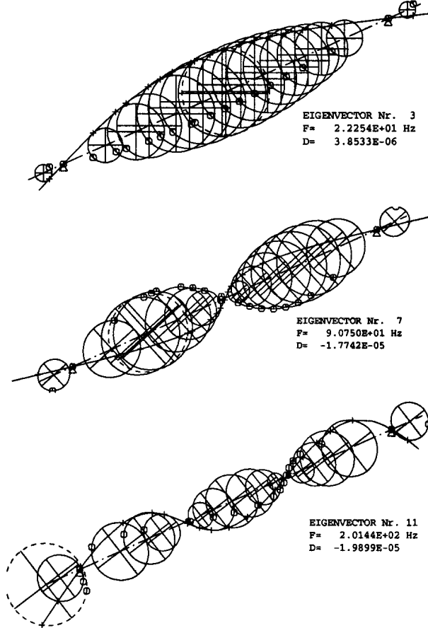
Figure 46. Calculated Eigenmodes in Air.
