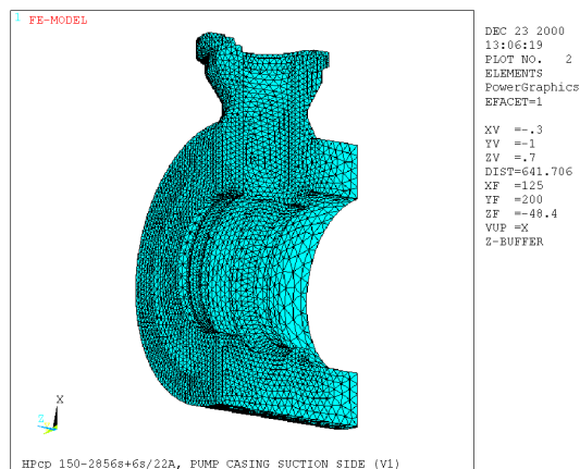
Figure 28. Analysis Model of Barrel End to Check Opening Compensation According to ASME Code.
