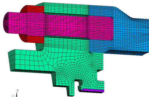
Figure 14. FE-Model of Cover and Bolted Connection with Barrel—Symmetry Is Used and 1/24th of Circumference Is Modeled.
