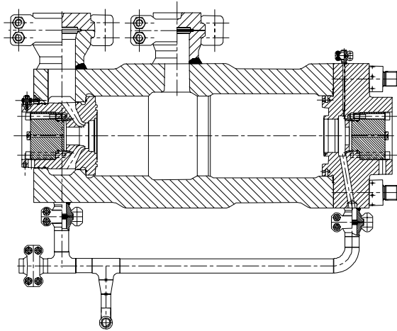
Figure 53. Hydrostatic Pressure Test Assembly.
