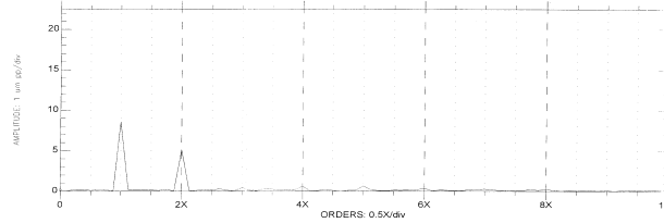
Figure 47. Frequency Spectrum at 6000 RPM and 331 M 3 /H (1457 GPM) Rated Flow, New-Condition.
