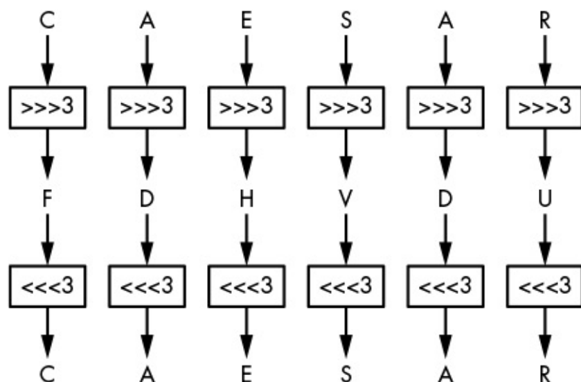
Figure 1-2: The Caesar cipher
