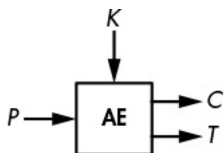
Figure 1-4: Authenticated encryption
