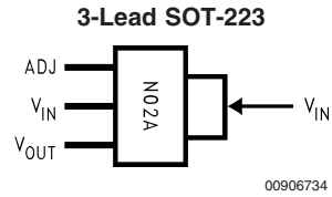
Front View Order Number LM337IMP Package Marked N02A See NS Package Number MP04A
