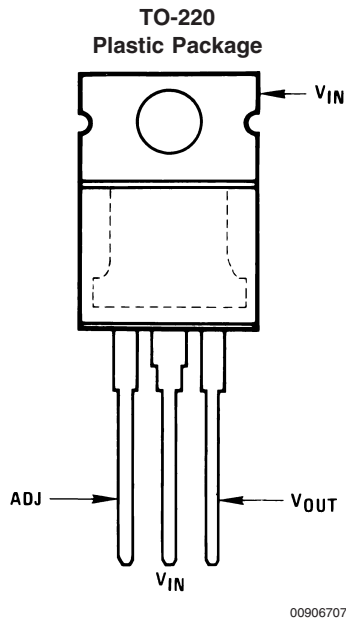
Front View Order Number LM337T See NS Package Number T03B
