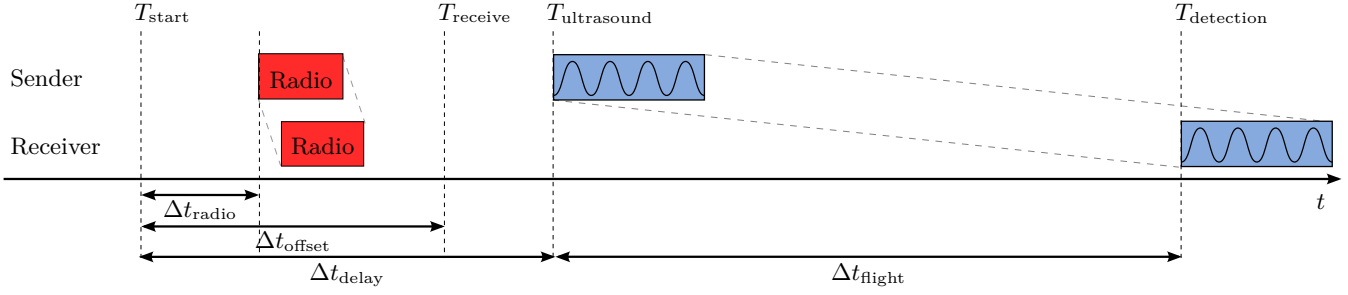
Figure 4: Timeline of events during a single ultrasound measurement between a sender and receiver node. The measurement is initiated by a radio packet, which is followed by an ultrasound pulse.
