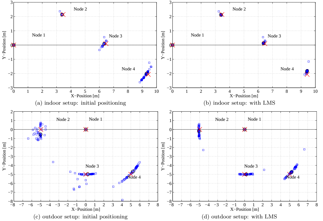
Figure 12: Experimental results for the indoor and outdoor settings: Initial position estimates are based on the distance and angle to the closest neighbor (plots (a) and (c)). Post-processing of position estimates is done using the method of least mean squares (LMS) (plots (b) and (d)). The average position over all ultrasound measurements for each node is indicated with a circle, the cross marker indicates the node position measured using a reference tape.
