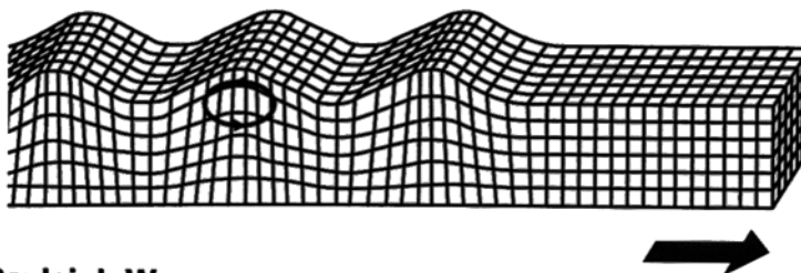
D. Rayleigh Wave
