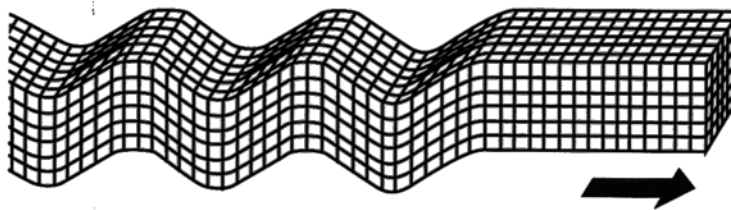
B. S Wave (SV wave shown for motion in vertical plane; SH wave similar but motion in horizontal plane)
