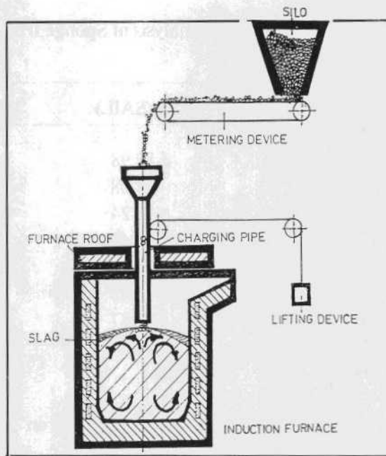
Fig.1 : Continuous charging method for direct reduced iron in to induction furnace
