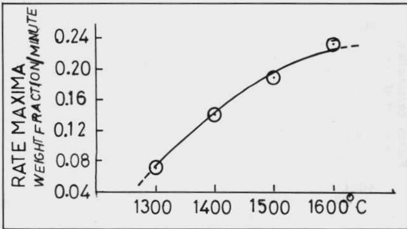
Fig.7 : Variation of the rate maxima with increasing temperature of molten pool in induction furnace
