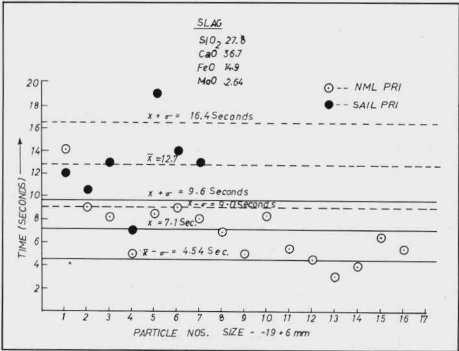
Fig.3 : Average melting time ( \bar{x} ) and standard deviation of NML and SAIL sponge iron in acidic slag at 1300 °C in medium frequency coreless induction furnace
