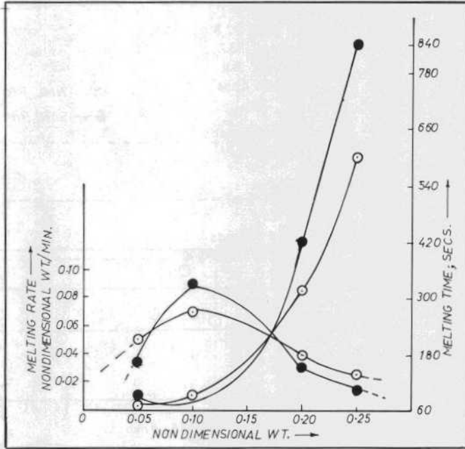
Fig.5: Optimisation of melting rate of sponge iron in molten iron (C-3.9, Si-1.7) 7.00 kg at 1300 °C in coreless induction furnace
