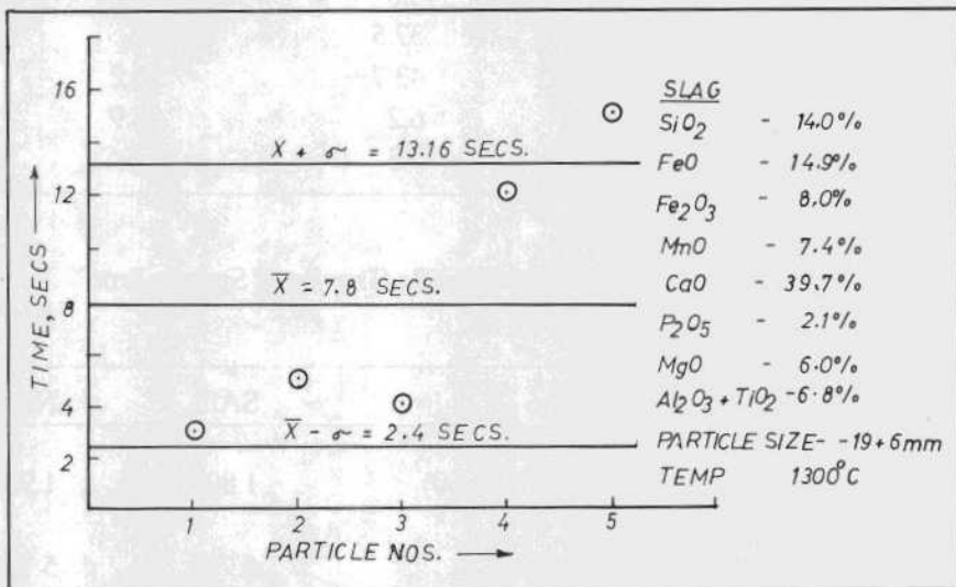
Fig.2 : Average melting time and standard deviations ( \sigma ) of NML sponge iron basic slag at 1300 °C in medium frequency foreless induction furnace
