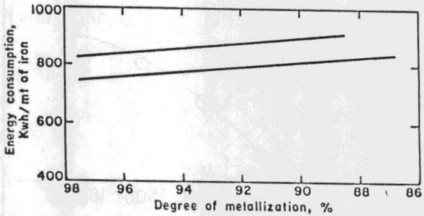
Fig. 9 : Effect of the degree of reduction of DRI on the energy consumption during batch melting in a coreless induction furnace
