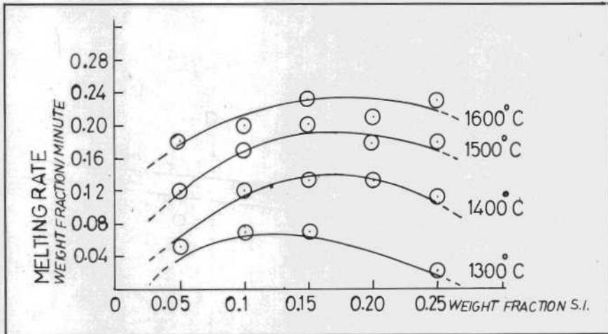
Fig.6 : Optimisation of melting rate of sponge iron in molten metal (C, 3.5 - 4.5, Si, 1.7-1.9) pool at different temperatures
