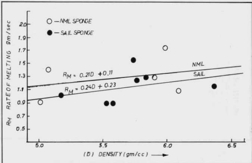
Fig.4 : Regression of rate of melting upon density in basic slag at 1300 °C
