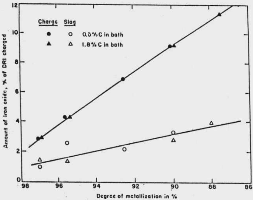
Fig.8 : Effect of the degree of metallization of DRI on the amount of the iron oxide in the charge and in the slag, expressed as % of the DRI charged
