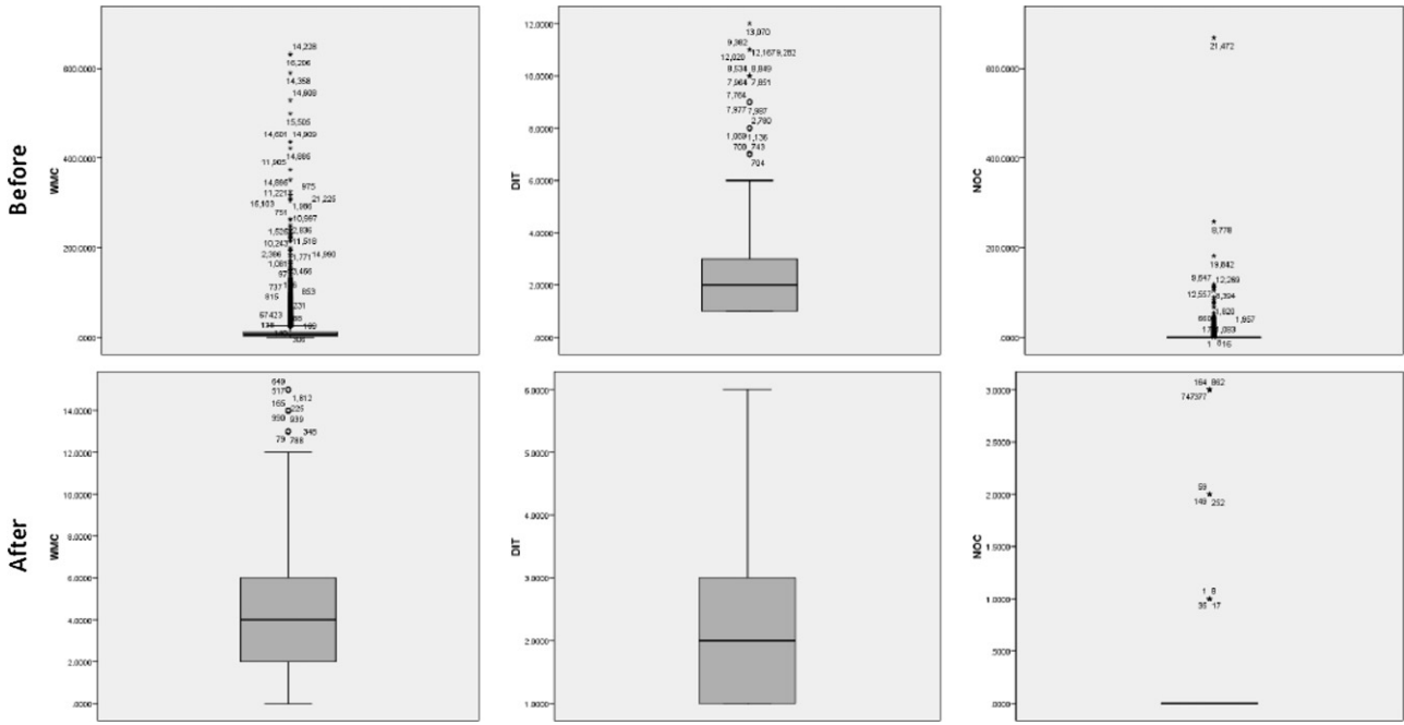
Fig. 4. Boxplots of WMC, DIT and NOC before and after outlier elimination.
