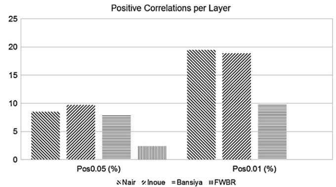
Fig. 8. Percentages of positive correlations per layer and per project to the reuse metrics.
