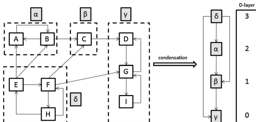
Fig. 1. Classycle acyclic digraph creation (Elmer, 2011).
