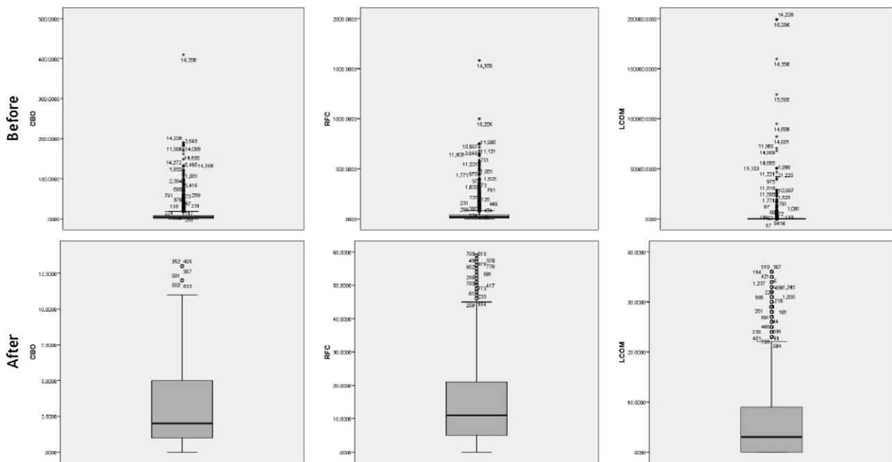
Fig. 5. Boxplots of CBO, RFC and LCOM before and after outlier elimination.
