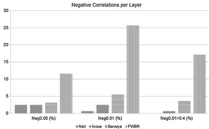
Fig. 7. Percentages of negative correlations per layer and per project to the reuse metrics.
