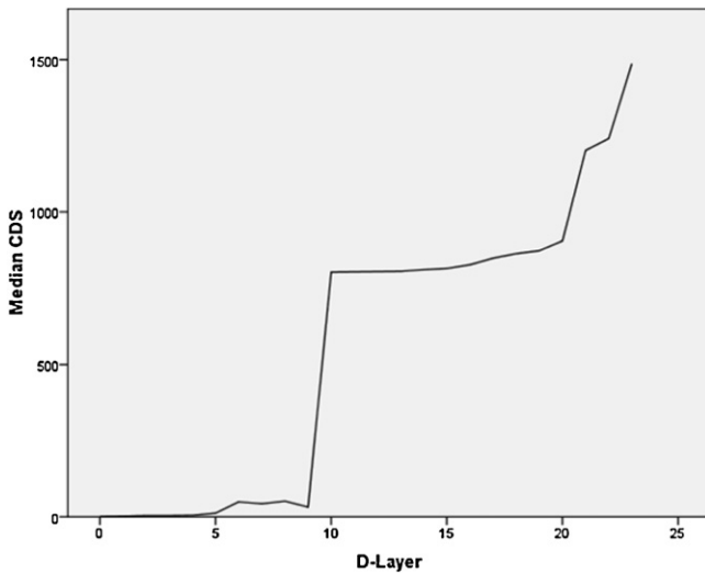
Fig. 6. CDS median per D-layer.
