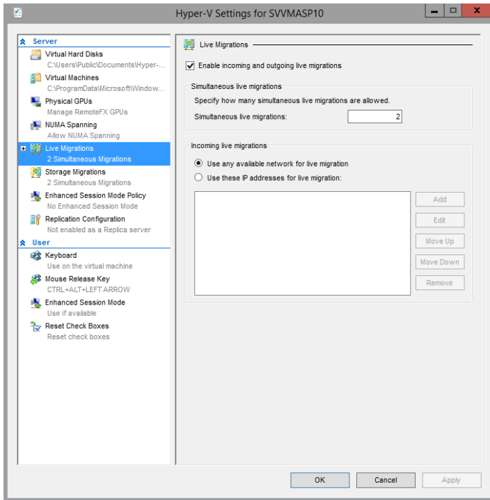
Figure 2-11: Live migration settings for a host
