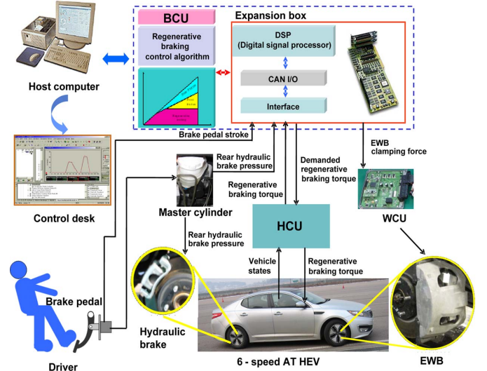
Fig. 10. Configuration of the vehicle test apparatus.
