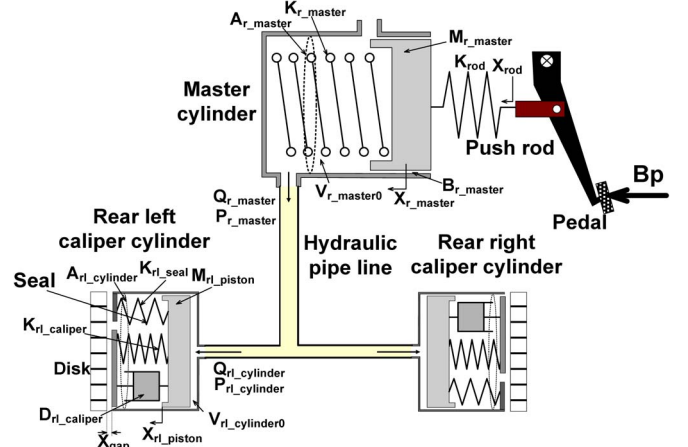
Fig. 4. Rear hydraulic brake model.
