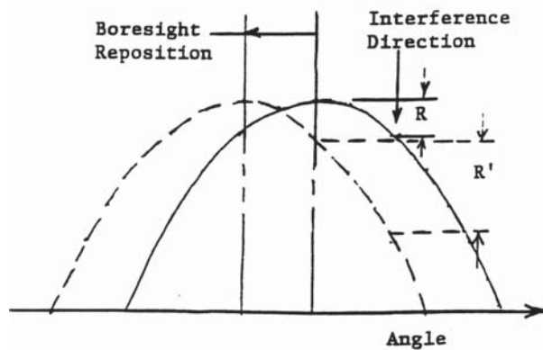
Figure 6-8 Contour and pattern description of adaptive beam repositioning [22] © 1996 IEEE)
