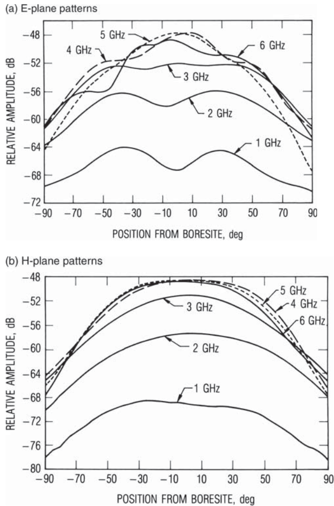
Figure 7-8 Principal plane patterns for microstrip antenna [22] © 1992 IEEE)
