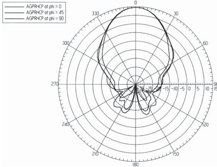
(b) Measured diagonal plane pattern
