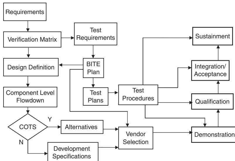
Figure 9-4 The overall user segment test process
