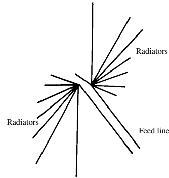
spiderweb antenna
