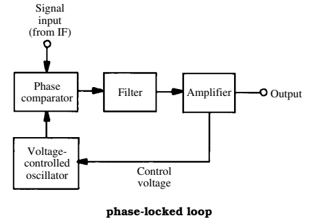
phase-locked loop
