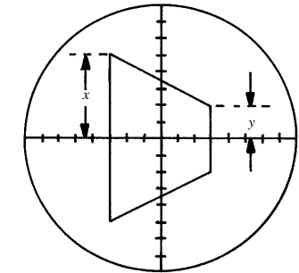
trapezoidal pattern
