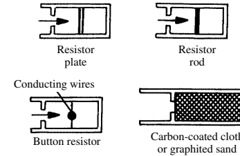
waveguide dummy load
