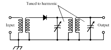
passive frequency multiplier
