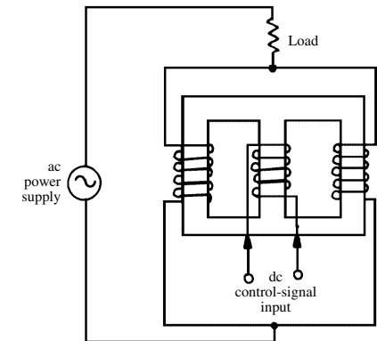
magnetic amplifier
