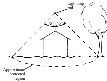
cone of protection
