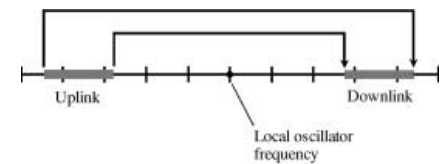
inverting transponder
