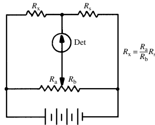
ratio-arm bridge
