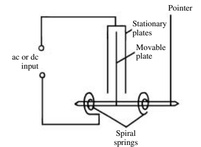
Kelvin absolute electrometer
