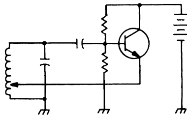
Hartley oscillator
