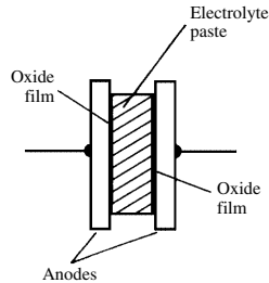
nonpolarized electrolytic capacitor
