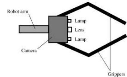
eye-in-hand system
