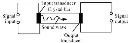
acoustic delay line
