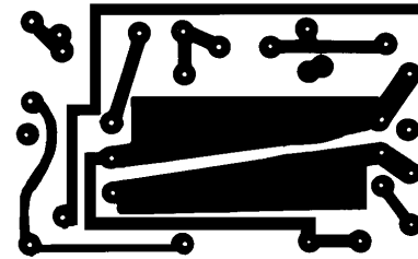
printed-circuit template
