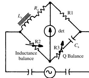
Hay bridge
