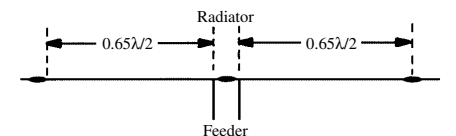
double-extended Zepp antenna
