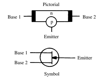
unijunction transistor
