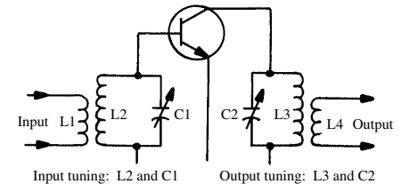
double-tuned circuit
