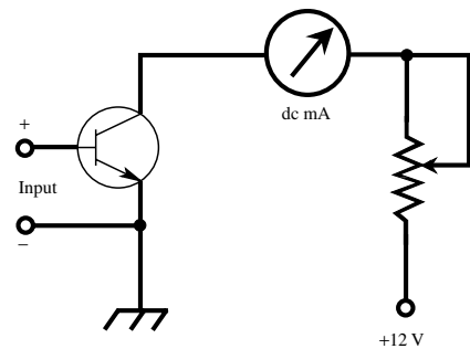
electronic current meter
