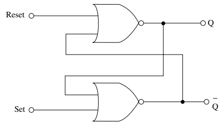
bistable multivibrator
