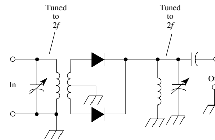
frequency doubler
