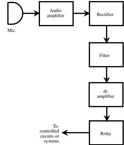
sound-operated relay
