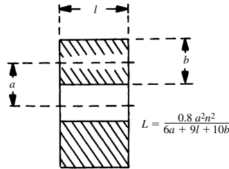
Wheeler's formula (dimensions illustrated)
