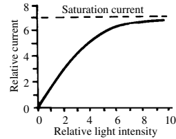
photovoltaic cell
