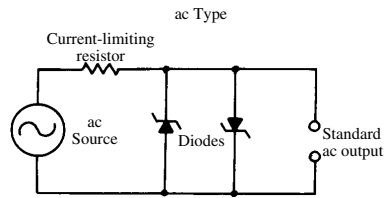
zener-diode voltage reference
