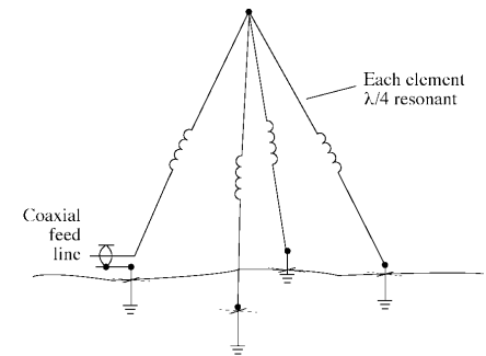
Alexanderson antenna
