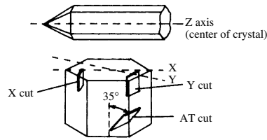
crystal cuts
