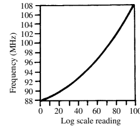
calibration curve
