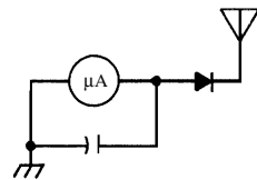
field-strength meter
