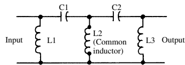
common-inductor coupling
