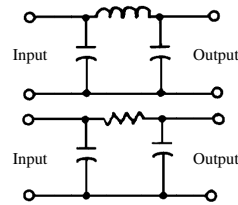
pi filters
