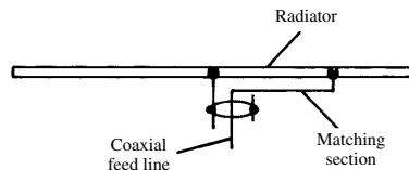
gamma match
