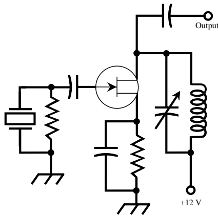
Miller oscillator
