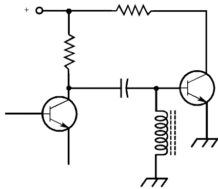
zero-bias operation
