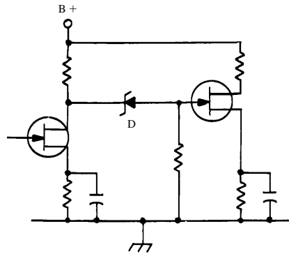
zener-diode coupling element
