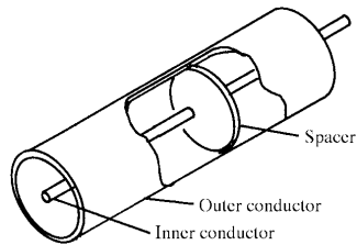
air-dielectric coax
