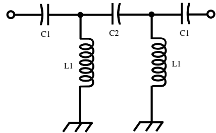
bilateral network
