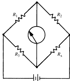
Wheatstone bridge
