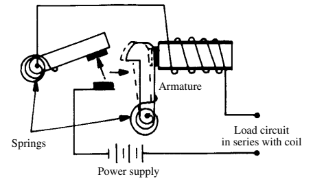
circuit breaker
