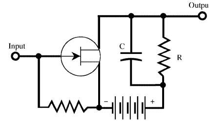
active RC network
