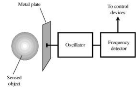
capacitive proximity sensor
