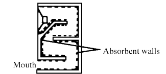
acoustic labyrinth
