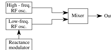
subcarrier frequency modulation
