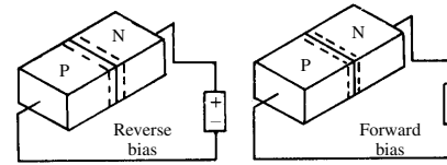
biased diodes
