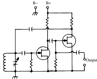
Franklin oscillator
