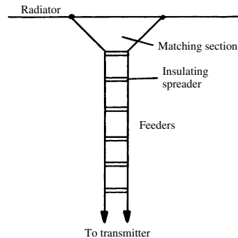
wye-matched-impedance antenna
