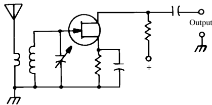
preamplifier
