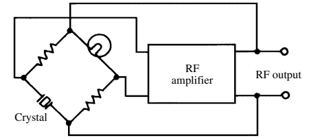
Meacham oscillator
