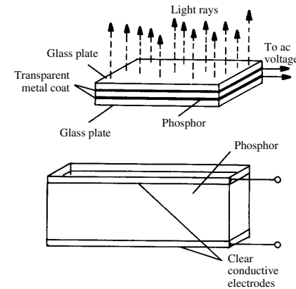
electroluminescent cell
