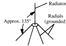
drooping radials
