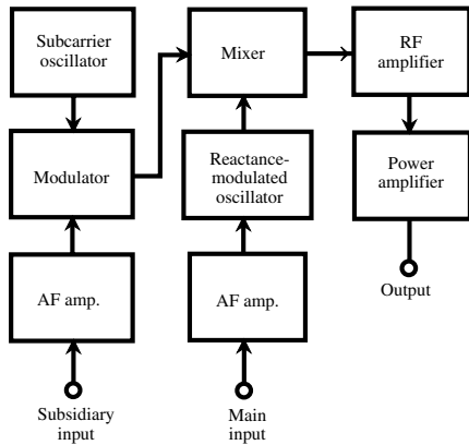
multiplexing, 1.
