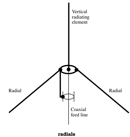
radials
