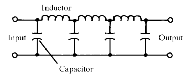
artificial transmission line
