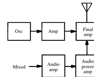
high-level modulation
