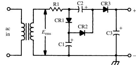
tripler, 1
