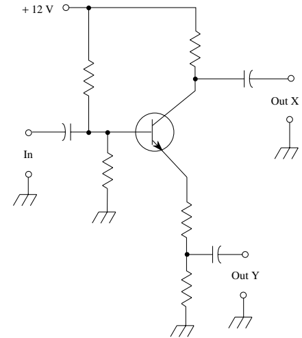
paraphase inverter
