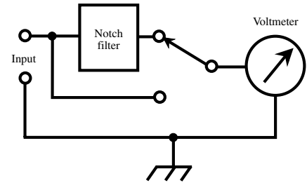
distortion meter
