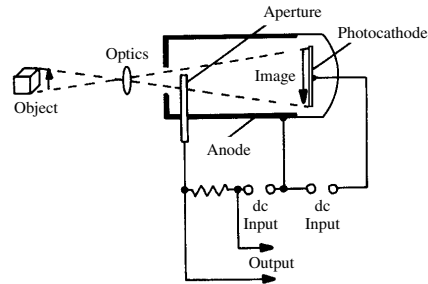
dissector tube
