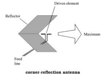
corner-reflection antenna
