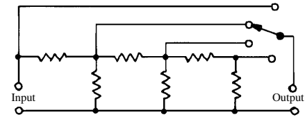
ladder-type attenuator
