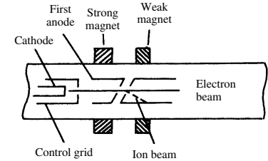
slashed-field-gun CRT
