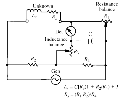
Anderson bridge
