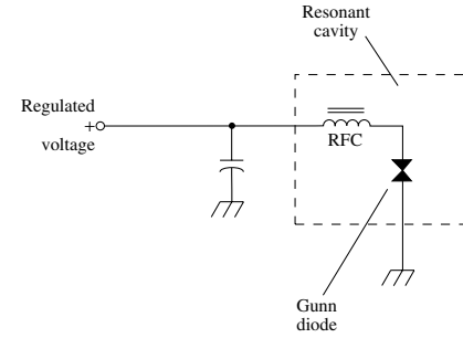
diode oscillator, 1
