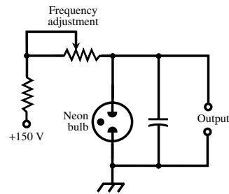
neon-bulb oscillator
