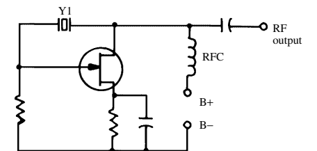
Pierce oscillator
