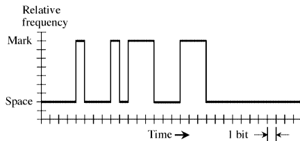
frequency-shift keying
