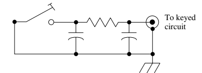
spark suppressor
