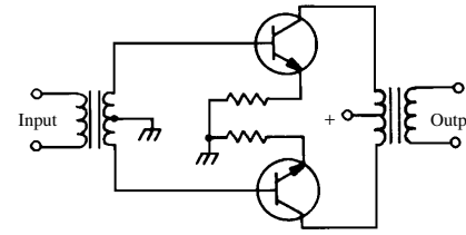
power amplifier
