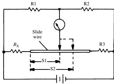
Carey-Foster bridge
