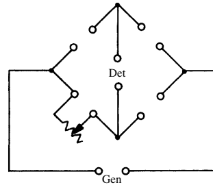
skeleton bridge
