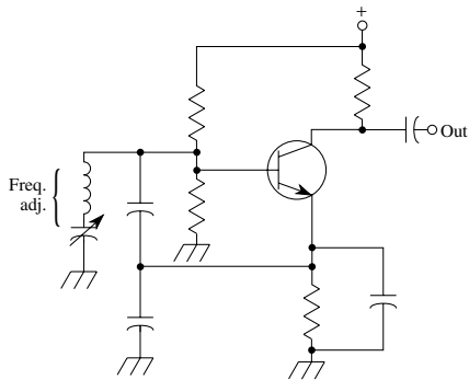
Clapp oscillator
