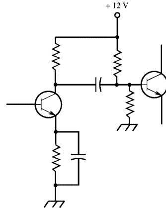
bypass capacitor
