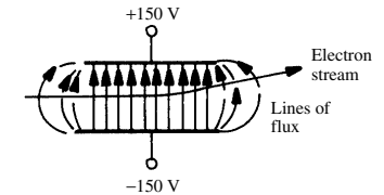
electrostatic deflection
