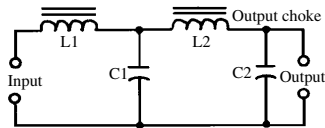
output choke
