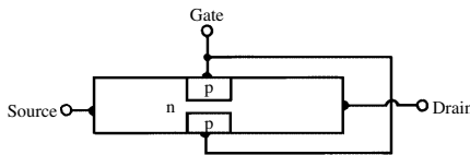
n-channel junction field-effect transistor
