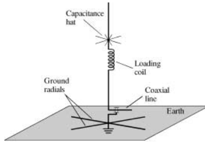
inductive loading
