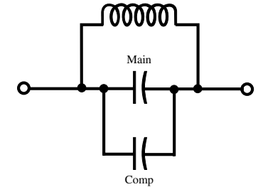
compensating capacitor, 1.
