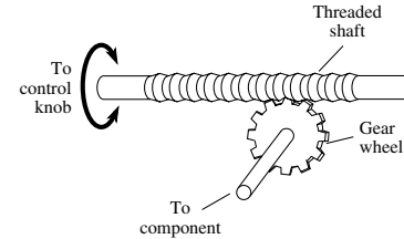
worm drive
