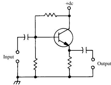
emitter follower
