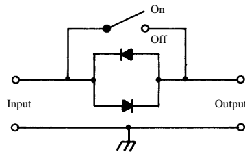
threshold detector
