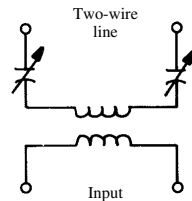
series antenna tuning
