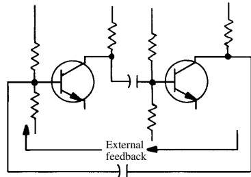
external feedback
