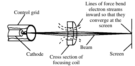
electromagnetic focusing
