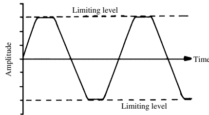
peak limiting
