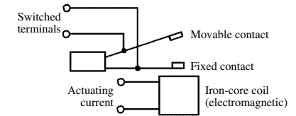
electromechanical relay
