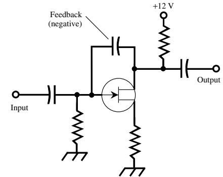
feedback, 1.
