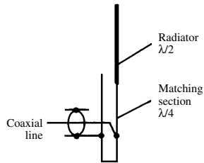
J antenna
