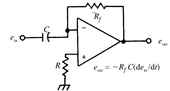
analog differentiator
