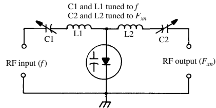
varactor frequency multiplier
