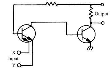
transistor-transistor logic
