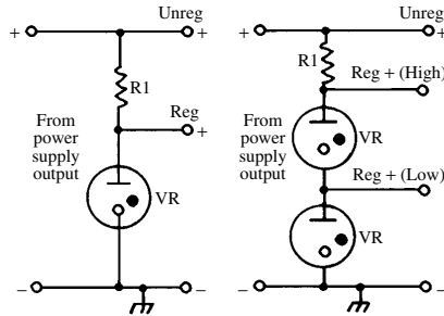
L-type voltage regulator
