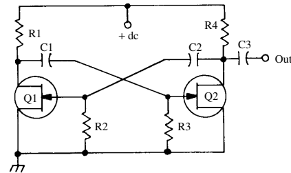
drain-coupled multivibrator
