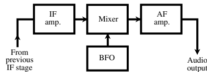
beat-frequency oscillator
