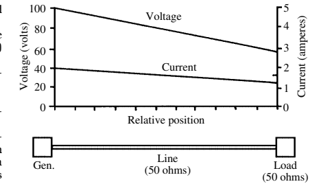
matched transmission line
