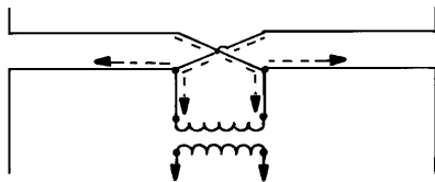
Adcock antenna
