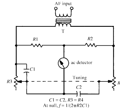
audio-frequency meter
