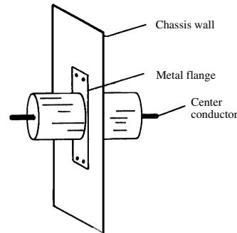
feedthrough capacitor
