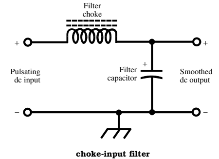
choke-input filter
