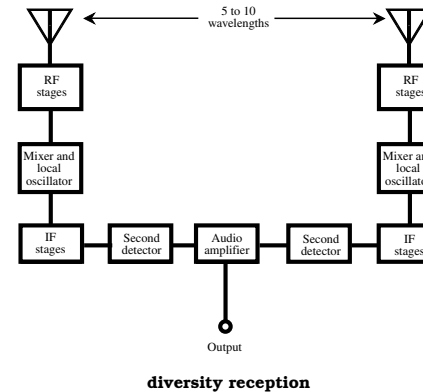
diversity reception
