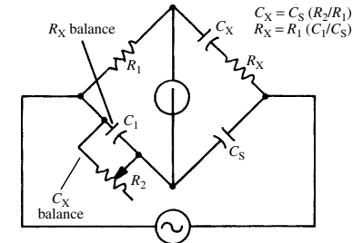
Schering bridge
