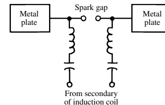
Hertz oscillator
