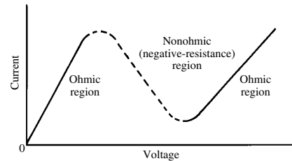
ohmic region
