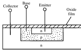
planar transistor
