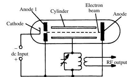
Heil oscillator
