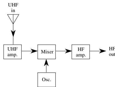
UHF converter, 1
