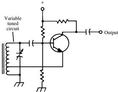
oscillator tuning
