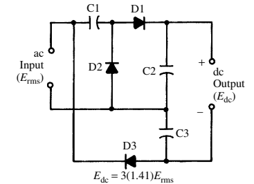
voltage tripler
