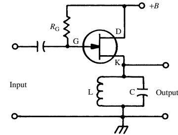
shock-excited oscillator
