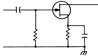
self-bias
