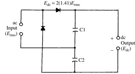
voltage doubler
