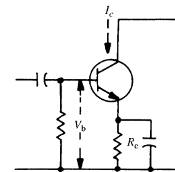
automatic bias
