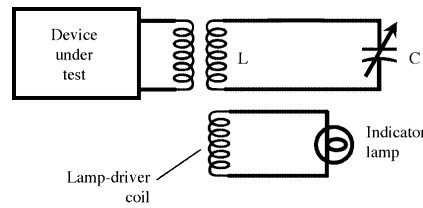
absorption wavemeter
