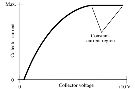
constant-current curve
