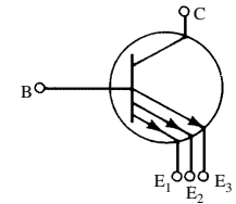
pentode transistor
