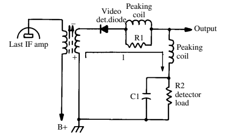
video detector
