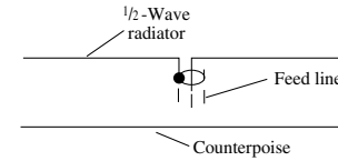
condenser antenna
