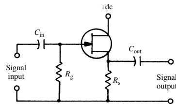
source follower
