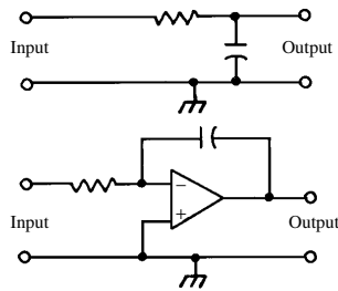
integrating networks
