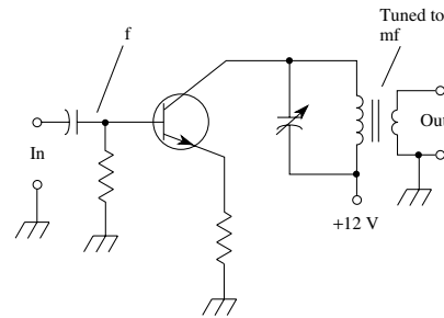
multiplier amplifier
