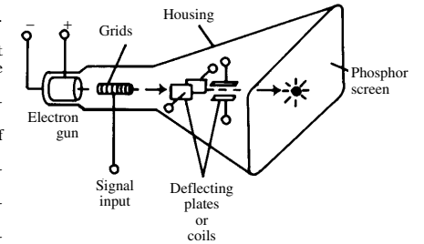
picture tube
