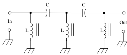
high-pass filter
