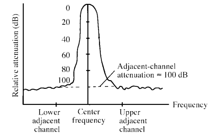
adjacent-channel attenuation
