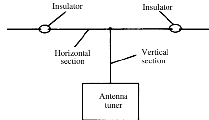
tee antenna
