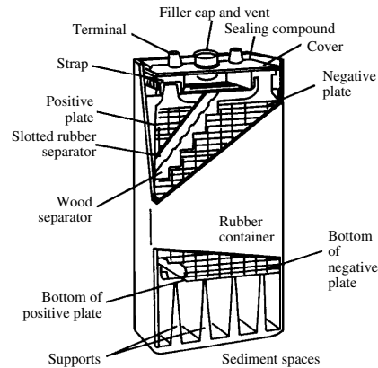
lead-acid cell
