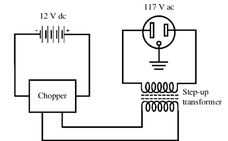
chopper power supply
