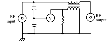
monimatch
