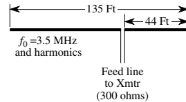
Windom antenna, 2
