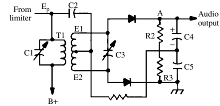
Foster-Seeley discriminator
