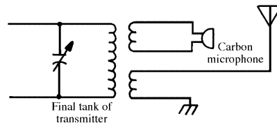
absorption modulation
