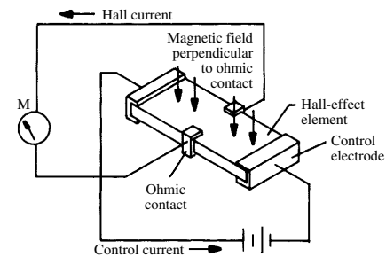
Hall generator
