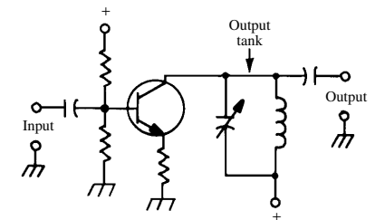
output tank
