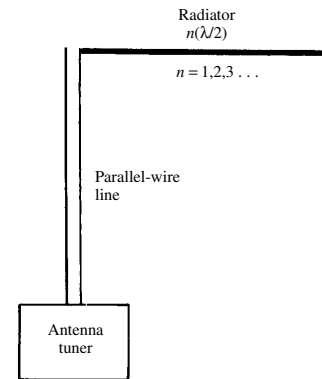
zeppelin antenna
