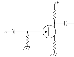
automatic gate bias
