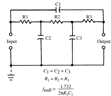
bridged integrator
