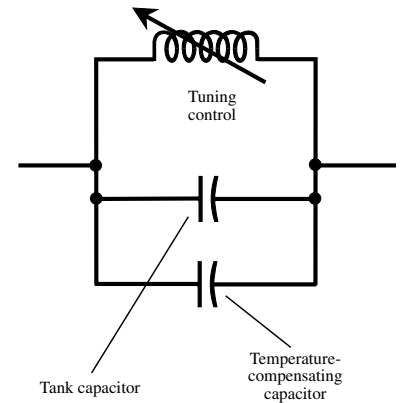
temperature-compensating component
