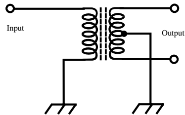
balanced output transformer, 2.
