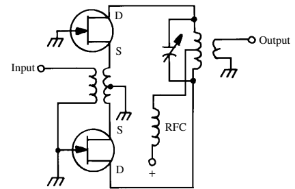
inverted amplifier
