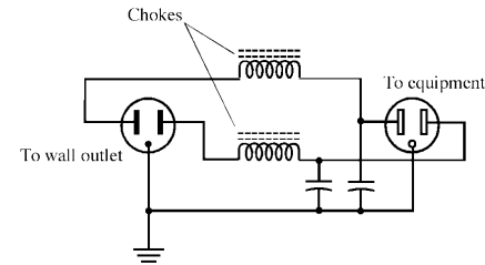
line filter
