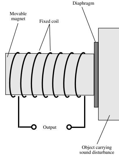
contact microphone
