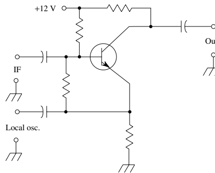
product detector
