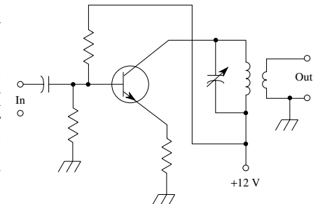
(General bipolar circuit)
