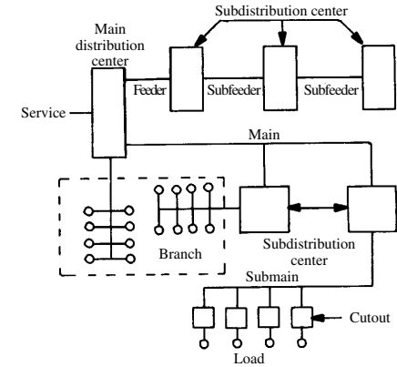
branch circuit (enclosed in broken lines)
