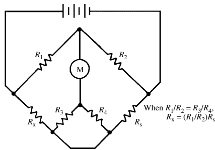
Kelvin double bridge
