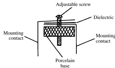
trimmer capacitor
