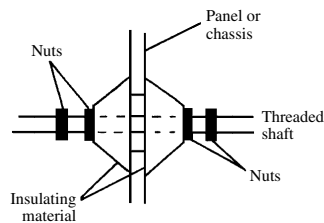
feedthrough insulator
