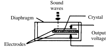
crystal microphones
