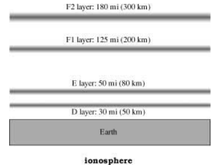
ionosphere
