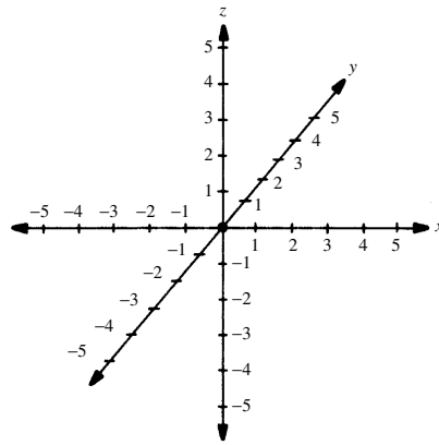
Cartesian three-space
