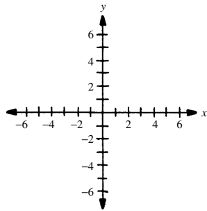
coordinate system (Cartesian)
