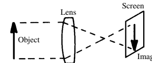
real image
