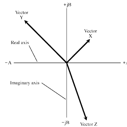
Argand diagram
