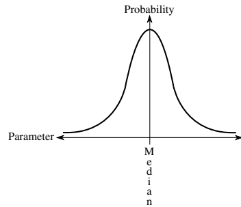
Gaussian distribution
