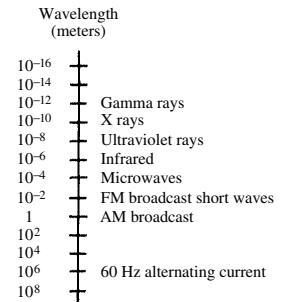
electromagnetic frequency spectrum
