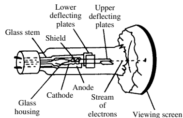
cathode-ray tube
