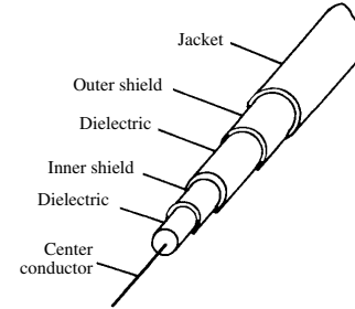
double shield
