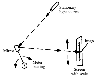
optical lever
