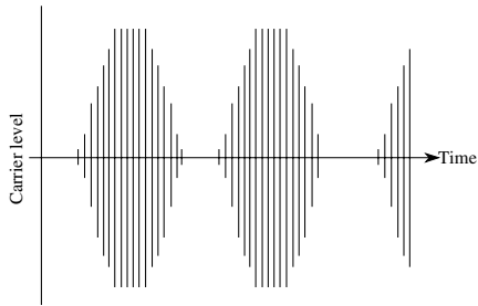
overmodulation
