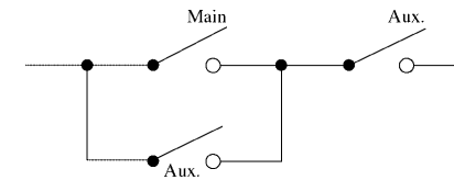
auxiliary switch, 2
