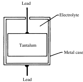
tantalum capacitor
