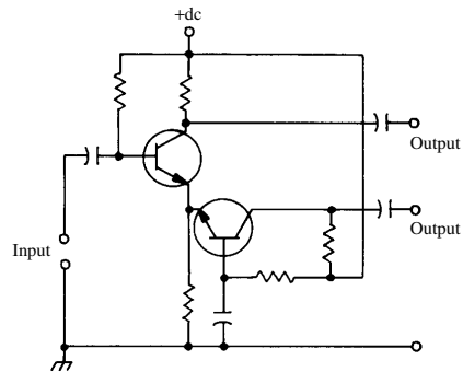
emitter-coupled phase inverter
