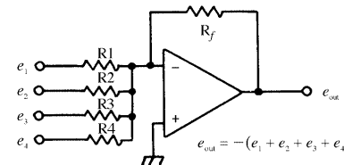
analog adder (inverting)
