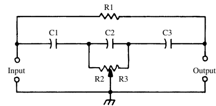
Hall network
