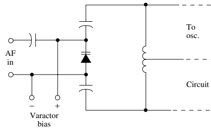
reactance modulator
