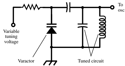
electric tuning
