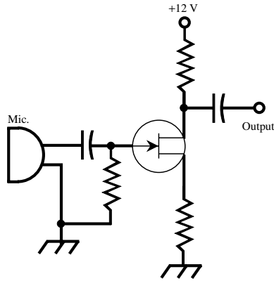
microphone amplifier
