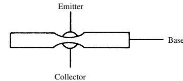
surface-barrier transistor
