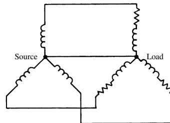
wye-wye circuit
