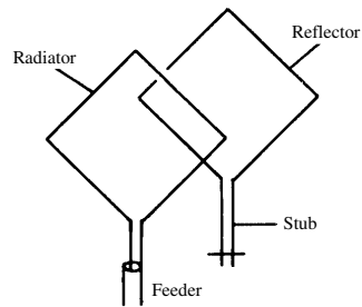
quad antenna
