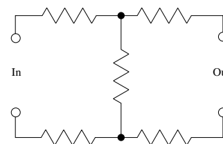
H network
