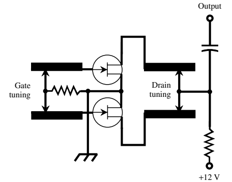
Meissner circuit
