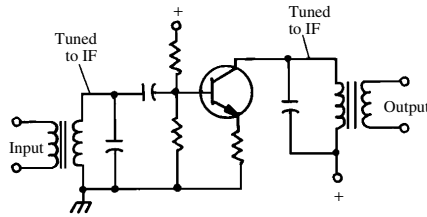
intermediate-frequency amplifier
