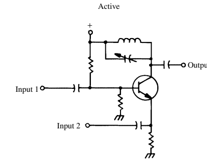
mixer
