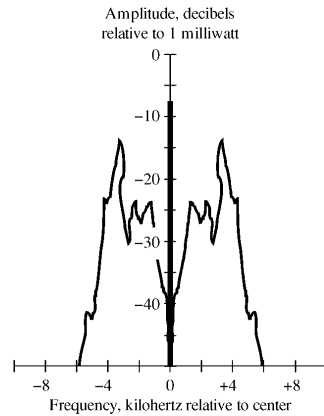
amplitude modulation
