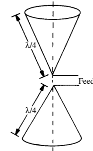
biconical antenna
