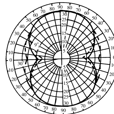
lobe (pattern of horizontal half-wave antenna)
