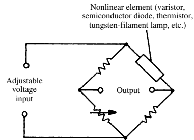
voltage-sensitive bridge
