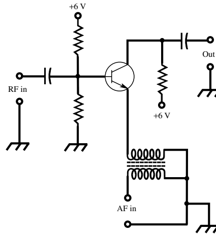
modulated amplifier
