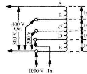
autotransformer
