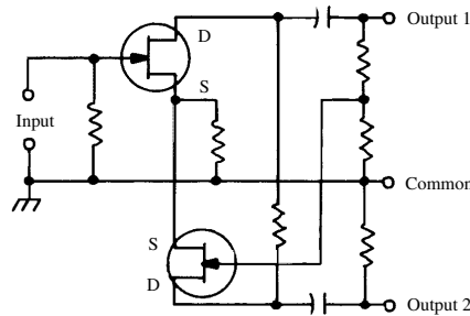
floating paraphase inverter
