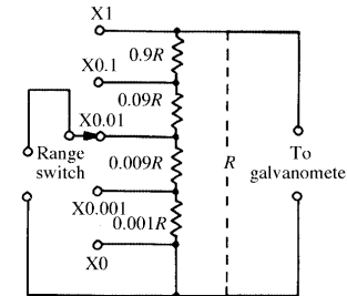
Ayrton-Mather galvanometer shunt
