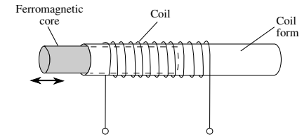
permeability tuning
