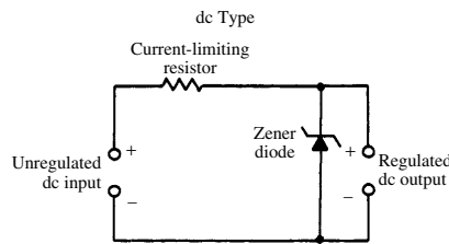
zener-diode voltage reference
