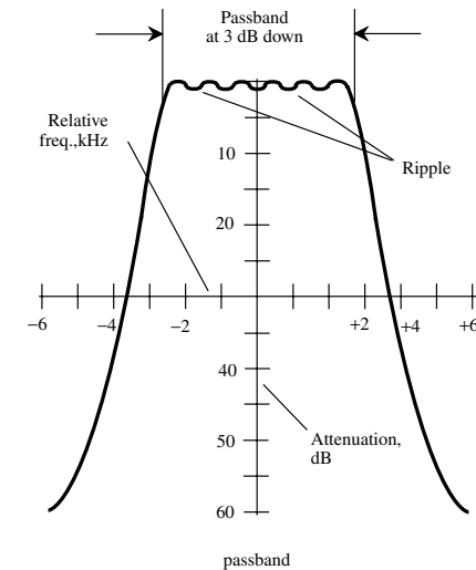
passband ripple
