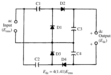
voltage quadrupler
