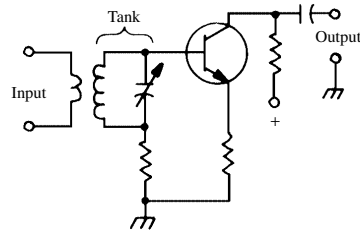
input tank
