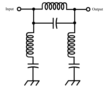
rejection filter
