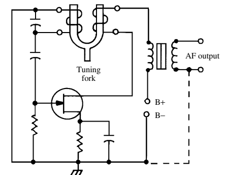
fork oscillator
