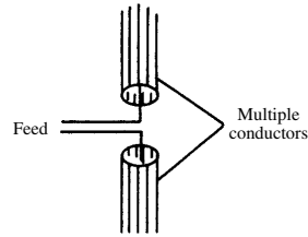
cage antenna
