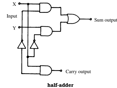
half-adder
