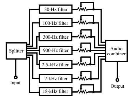
graphic equalizer
