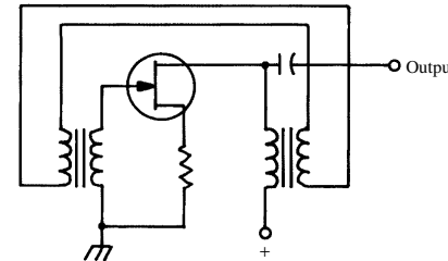
self-excited oscillator
