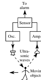
ultrasonic intrusion alarm
