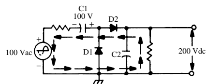
half-wave voltage doubler
