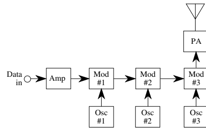
compound modulation
