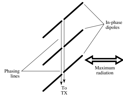
broadside array
