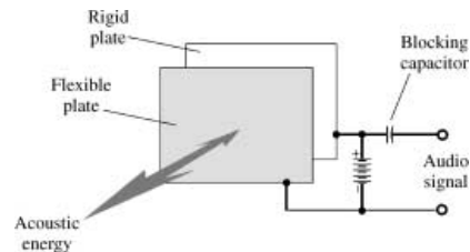
electrostatic speaker
