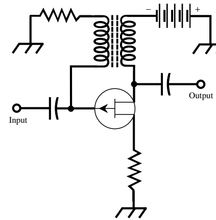
magnetic feedback
