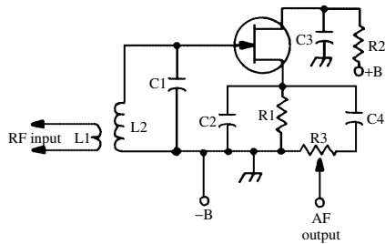
infinite-impedance detector
