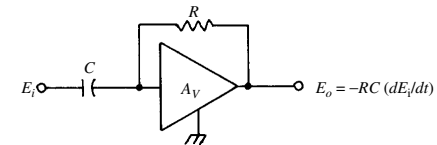
differentiator, 2
