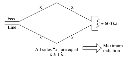
diamond antenna
