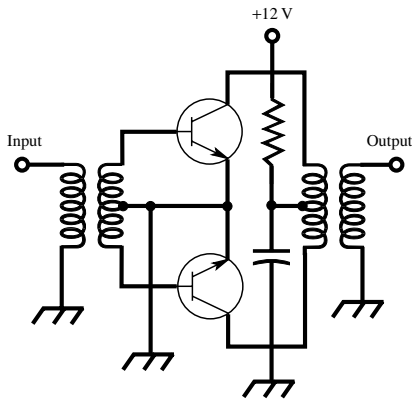
push-pull
