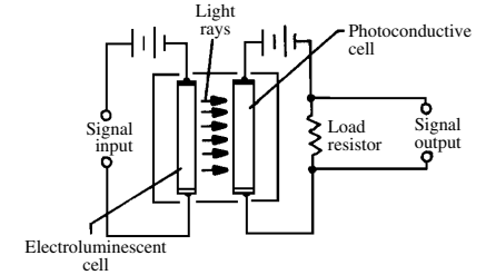
lumistor
