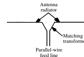
delta-matching transformer
