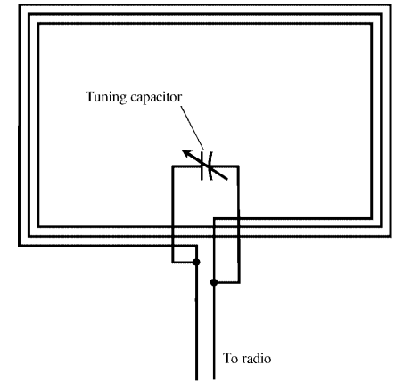
multiturn loop antenna
