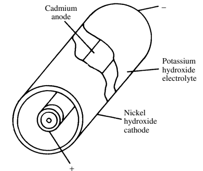
nickel-cadmium cell
