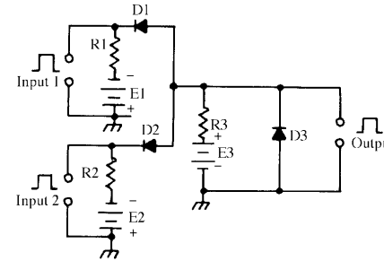
AND circuit
