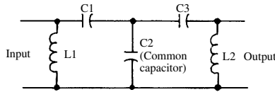
common-capacitor coupling
