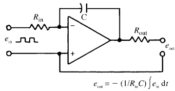
analog integrator
