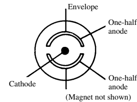
split-anode magnetron
