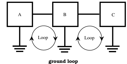
ground loop
