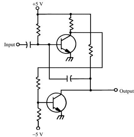
monostable multivibrator
