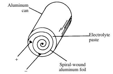
electrolytic capacitor
