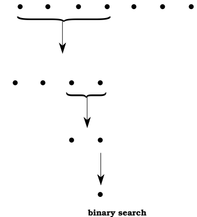
binary search
