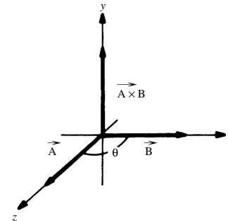
cross product
