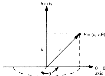
cylindrical coordinates
