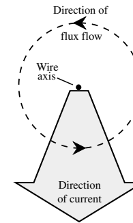
Ampere's Law
