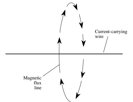
magnetic whirl
