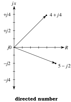
directed number
