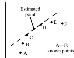
interpolation
