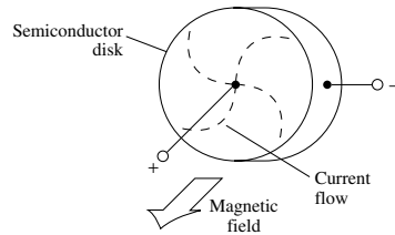
Corbino effect
