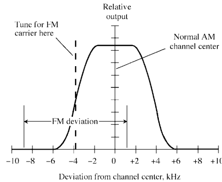
slope detector
