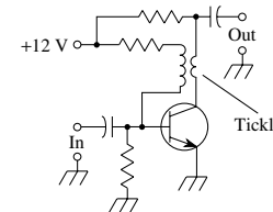
tickler-coil regeneration
