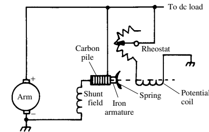
carbon-pile regulator
