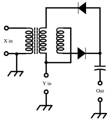
passive mixer
