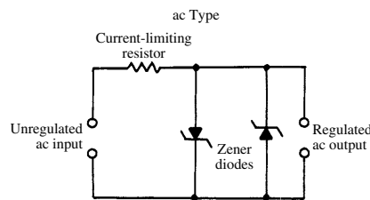
zener-diode voltage regulator
