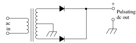
full-wave, center-tap rectifier
