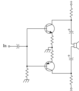
complementary-symmetry circuit
