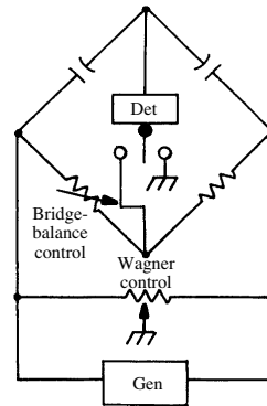
Wagner ground (with capacitance bridge)
