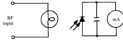
photoelectric wattmeter
