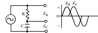
resistance-capacitance phase shifter
