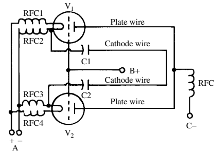
Kozanowski oscillator
