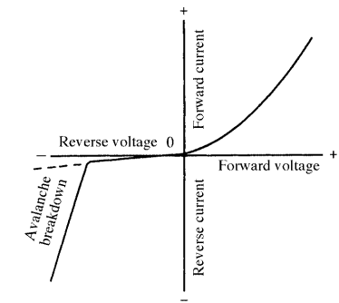
avalanche breakdown
