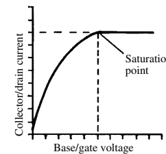
saturation point
