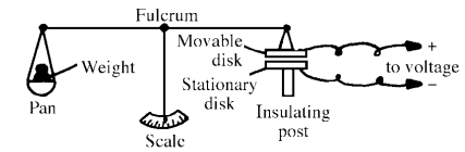
absolute measurement of voltage, 2
