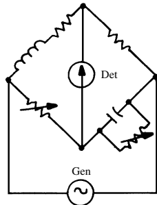
Maxwell bridge
