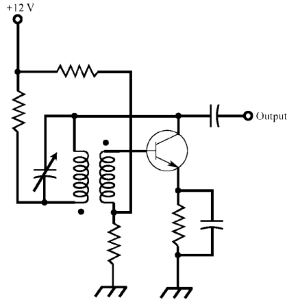
Armstrong oscillator
