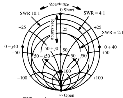
Smith chart
