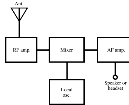
direct-conversion receiver
