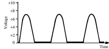
pulsating direct current
