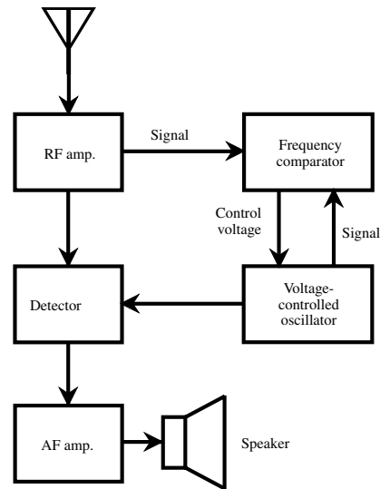
synchrodyne receiver
