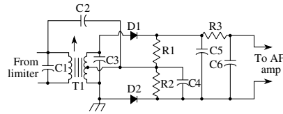
discriminator
