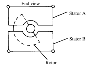
differential capacitor
