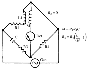
Carey-Foster mutual inductance bridge
