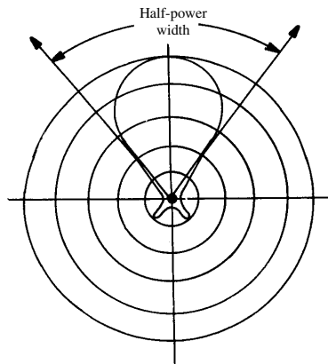
beamwidth of antenna
