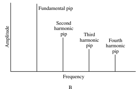
harmonic: waves (A) and spectrum-analyzer display (B)
