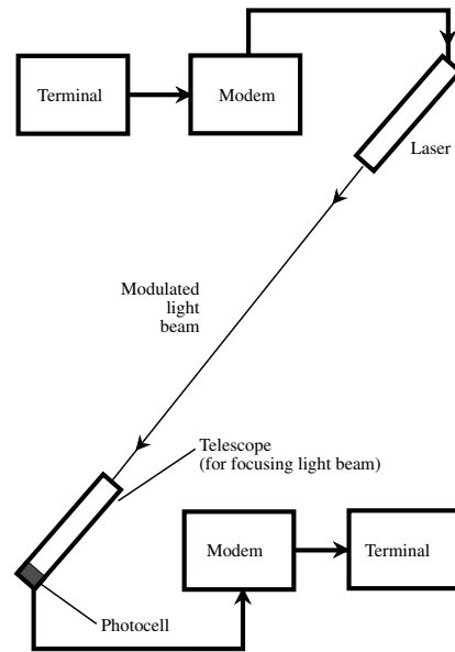
light-beam communication
