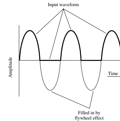
flywheel effect, 1.
