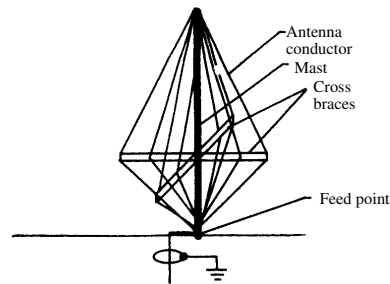
conical monopole antenna
