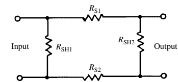
O network
