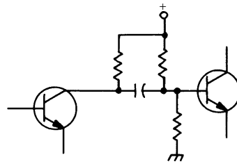
capacitive coupling
