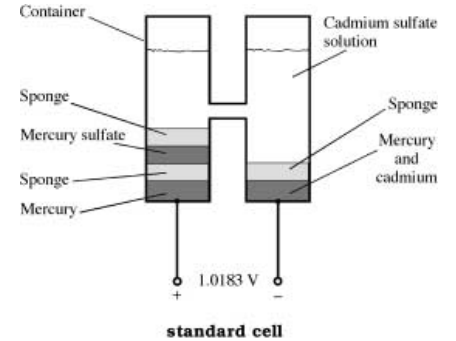
standard cell
