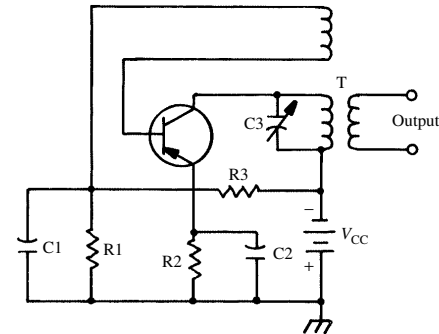
tuned-collector oscillator
