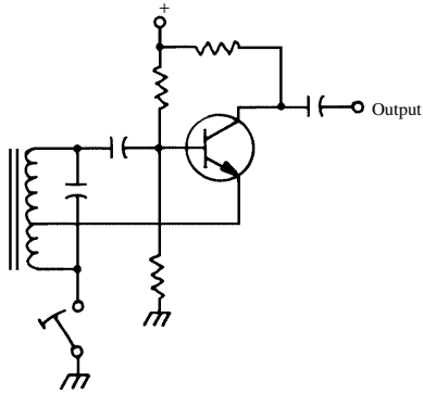
oscillator keying
