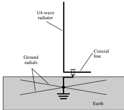
quarter-wave antenna
