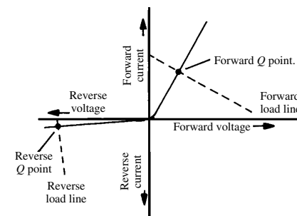
Q points on diode characteristic
