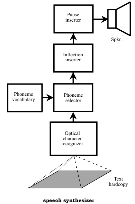
speech synthesizer
