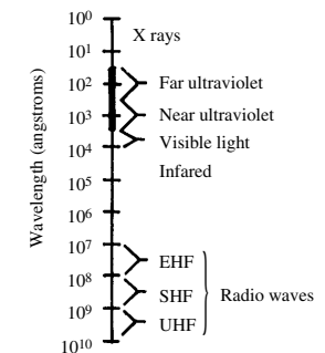
ultraviolet
