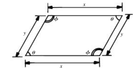
parallelogram
