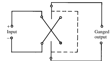
reversing switch
