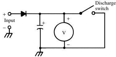
positive-peak voltmeter
