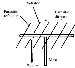
yagi antenna
