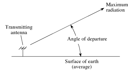
angle of departure
