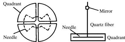
quadrant electrometer
