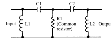
common-resistor coupling
