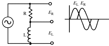
resistance-inductance phase shifter
