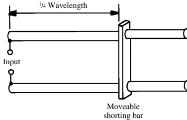
parallel-rod tuning
