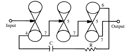
divide-by-seven circuit
