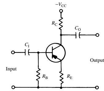
unbypassed emitter resistor ( R_E )
