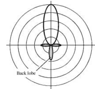
back lobe
