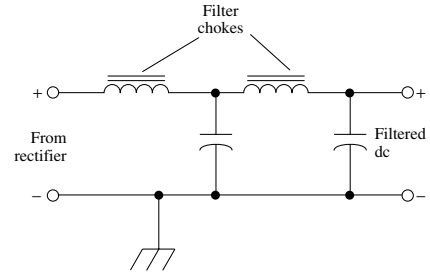
power-supply filter
