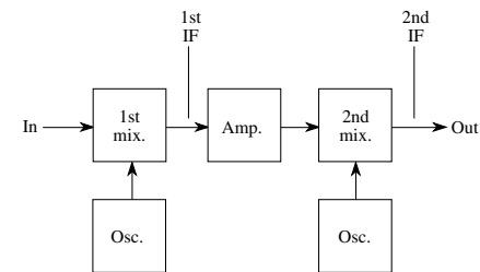
double conversion
