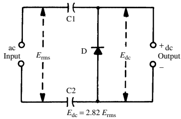
Villard circuit, 1
