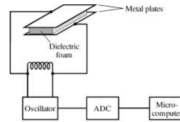
capacitive pressure sensor
