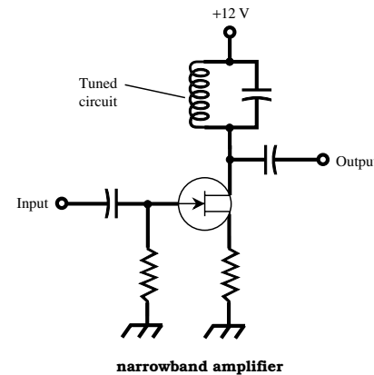
narrowband amplifier
