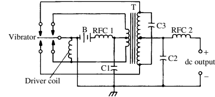
vibrator-type power supply
