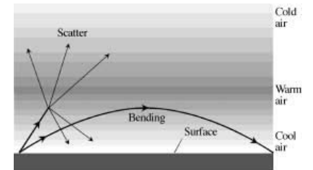
tropospheric propagation
