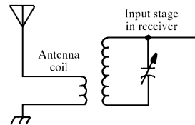
antenna coil
