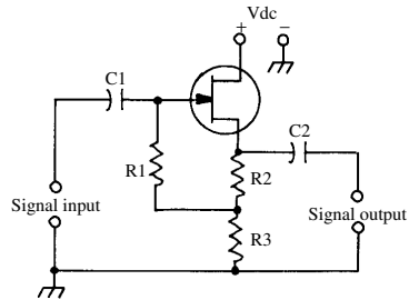
bootstrap circuit (with junction-type field-effect transistor)
