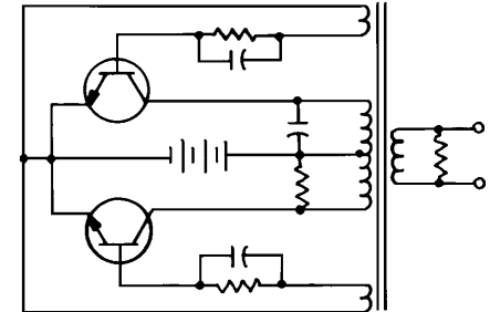
inverter, 1
