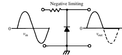
parallel limiter
