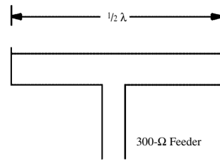
folded dipole
