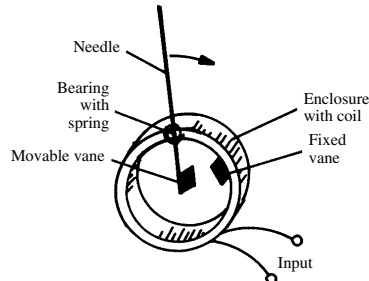
iron-vane meter
