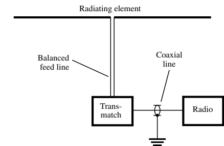
multiband antenna
