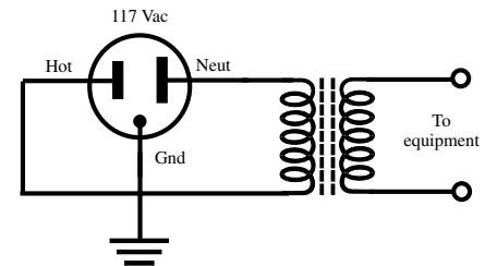
isolating transformer
