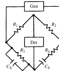
Wien bridge
