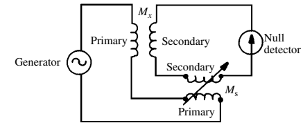
Felici mutual-inductance balance
