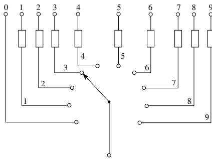
decade box
