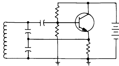
Colpitts oscillator
