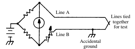
Varley loop bridge
