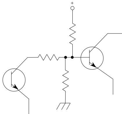
direct resistance coupling
