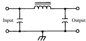
scratch filter
