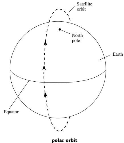
polar orbit
