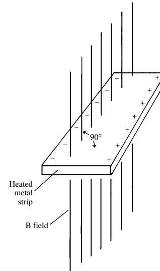
Nernst effect
