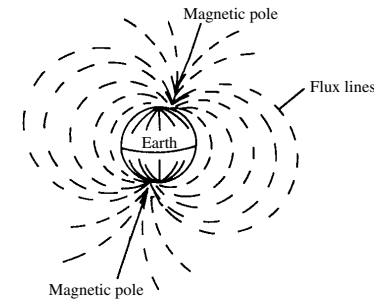
earth's magnetic field
