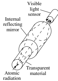
Cerenkov radiation
