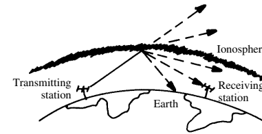
scattering
