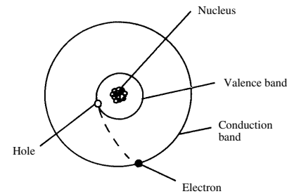
electron-hole pair
