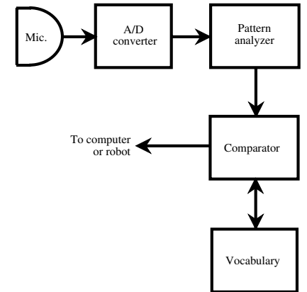
speech recognizer
