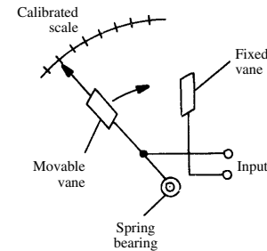
electrostatic voltmeter
