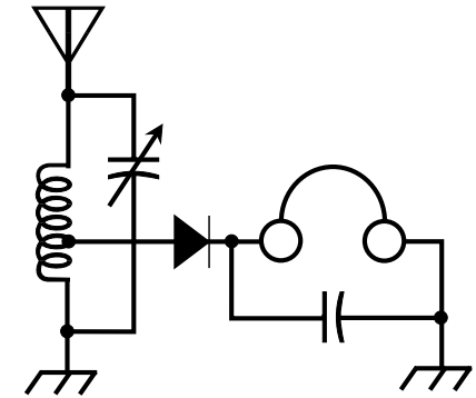
crystal set
