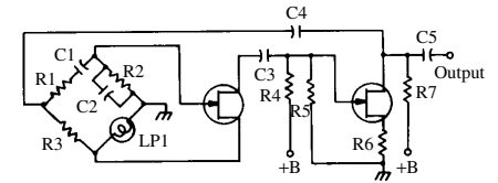
Wien-bridge oscillator
