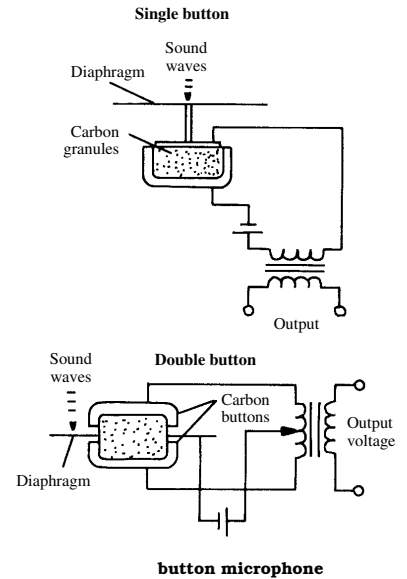
button microphone
