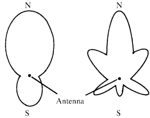
antenna patterns
