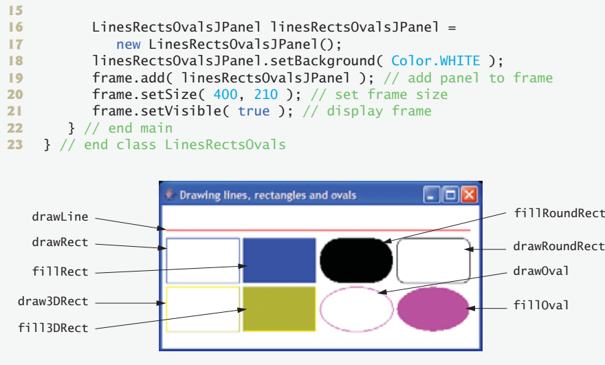
Fig. 12.19 | Creating JFrame to display lines, rectangles and ovals. (Part 2 of 2.)
