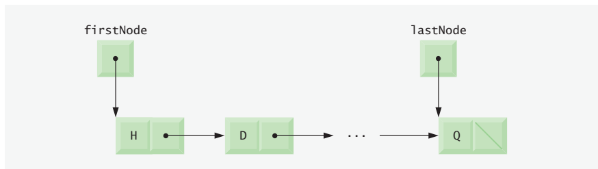
Fig. 17.2 | Linked list graphical representation.
