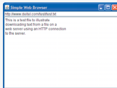
Fig. 24.4 | Test class for ReadServerFile. (Part 1 of 2.)
