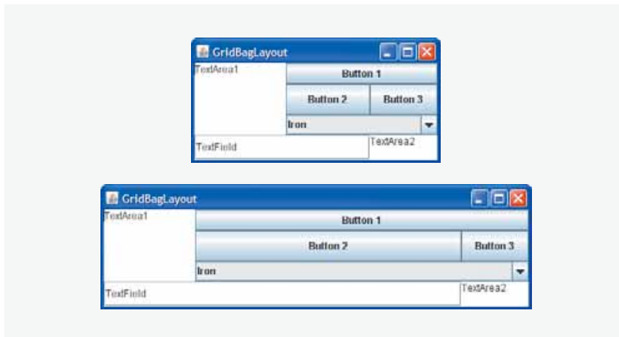
Fig. 22.20 | GridBagLayout with the weights set to zero.
