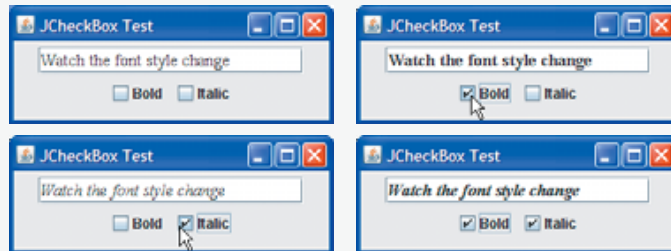
Fig. 11.18 | Test class for CheckBoxFrame.
