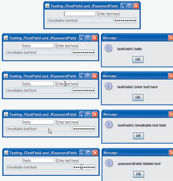
Fig. 11.10 | Test class for TextFieldFrame.
