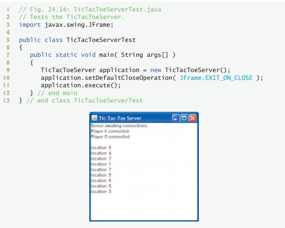
Fig. 24.14 | Class that tests Tic-Tac-Toe server.
