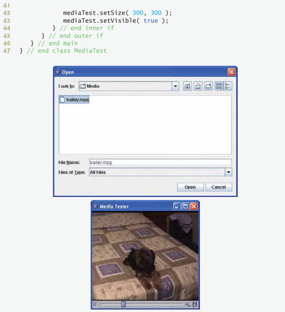
Fig. 21.7 | Test application that creates a MediaPanel from a user-selected file. (Part 2 of 2.)
