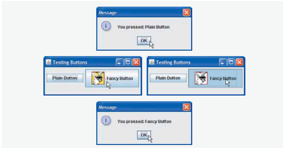
Fig. 11.16 | Test class for ButtonFrame. (Part 2 of 2.)
