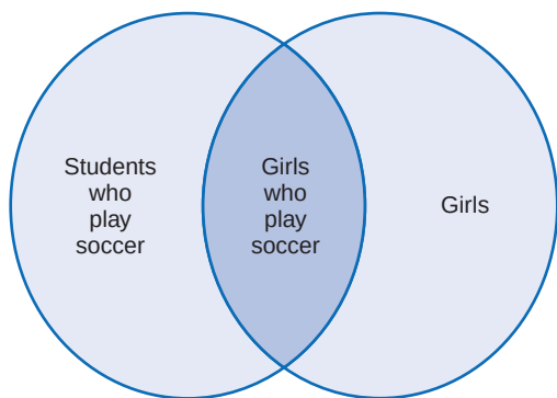
FIGURE 14-4 Venn diagram.
