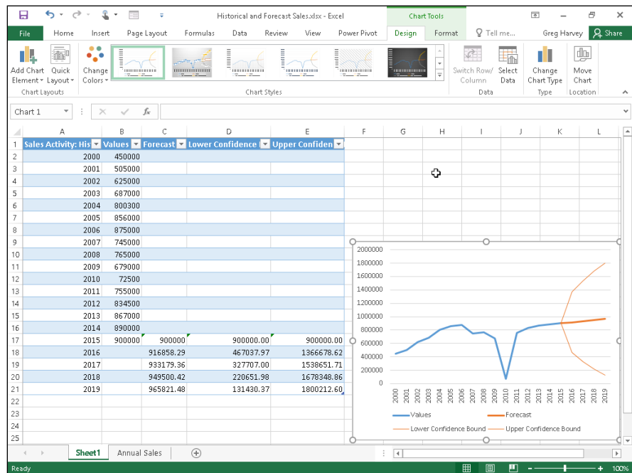
Figure 2-22: Worksheet with embedded line chart depicting historical and forecast sales created with the Forecast Sheet feature.
