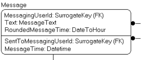
Figure 6-7. Messaging table before changing model to use surrogate key
