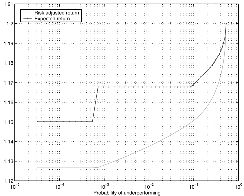
Figure 10. Trade-offs between probability of underperforming and returns.
