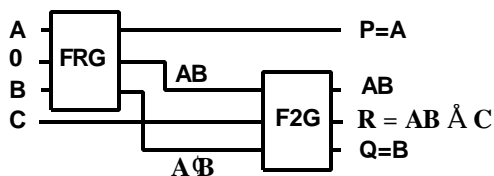
Fig. 8: Proposed parity preserving TG implementation using only two reversible gates
