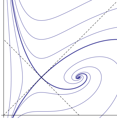
Figure 1. Phase portrait for a planar system with a hyperbolic fixed point (1, 1) together with the stable/unstable manifold (thick) and their linear counterparts (dashed).
