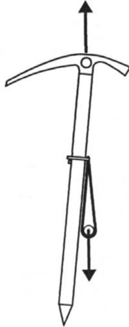
Strength test of the attachment device
