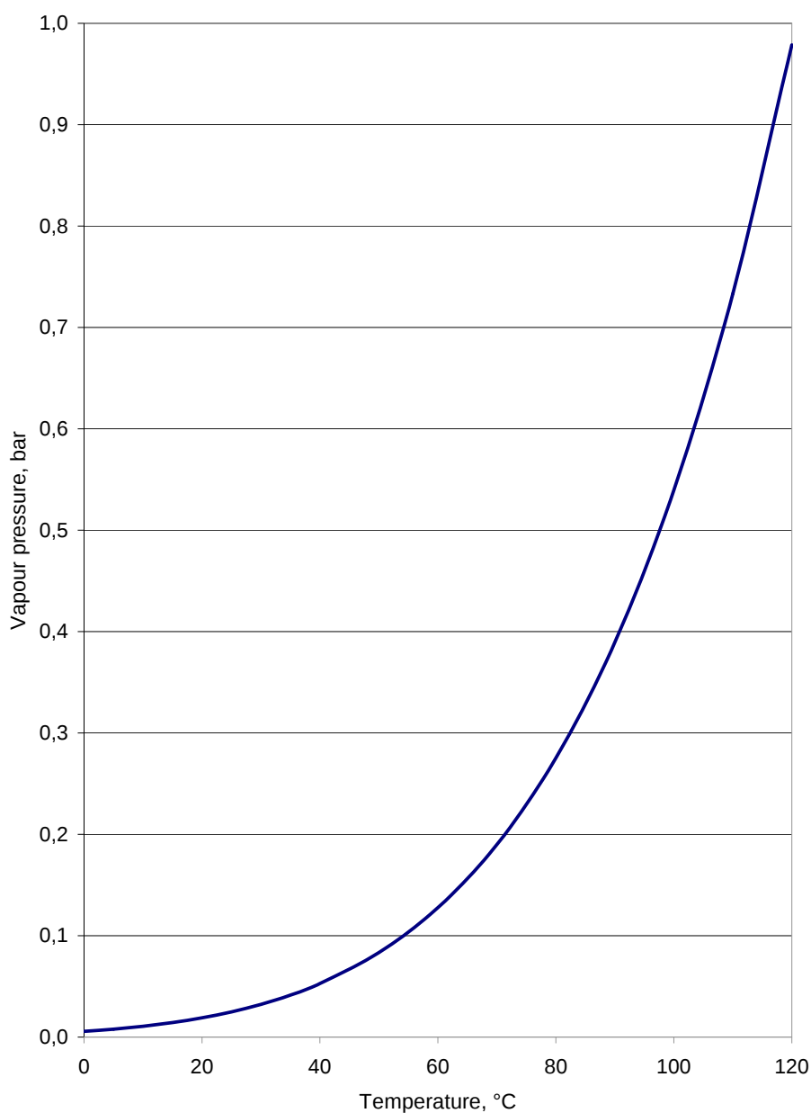
Vapour pressure of perchloroethylene
