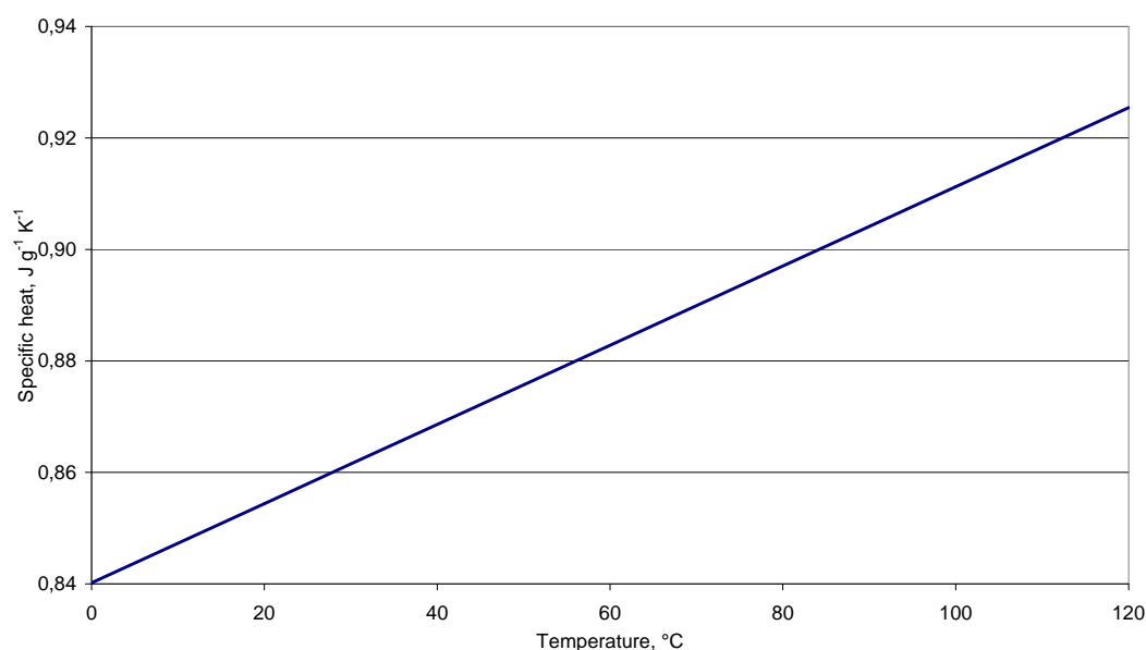
Specific heat of perchloroethylene
