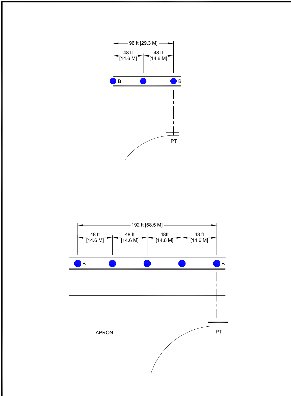
Figure H-14. Typical Single Straight Taxiway Edges (Less Than 200 ft (61 m)) (Legacy Figure 19)
