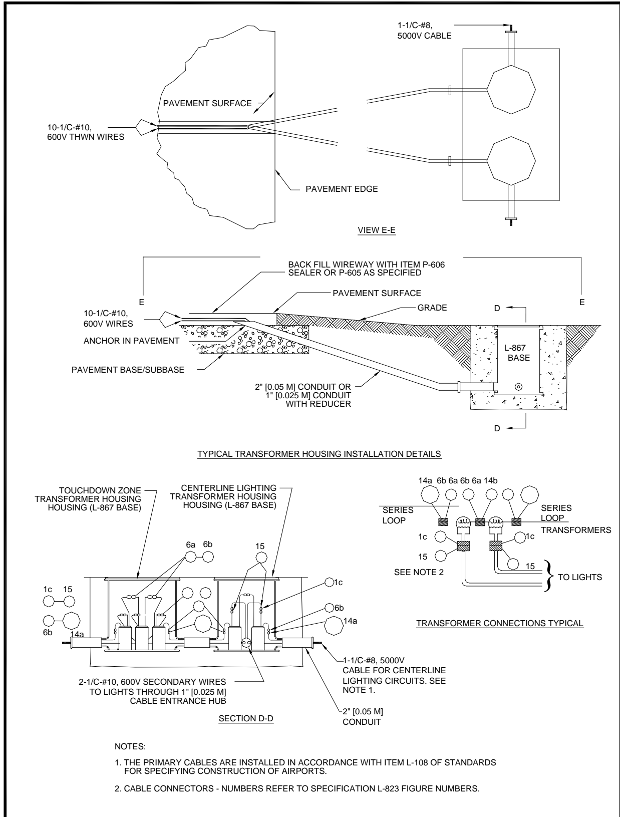
Figure A-41. Transformer Housing Installation Details Inset Type Lighting Fixtures
