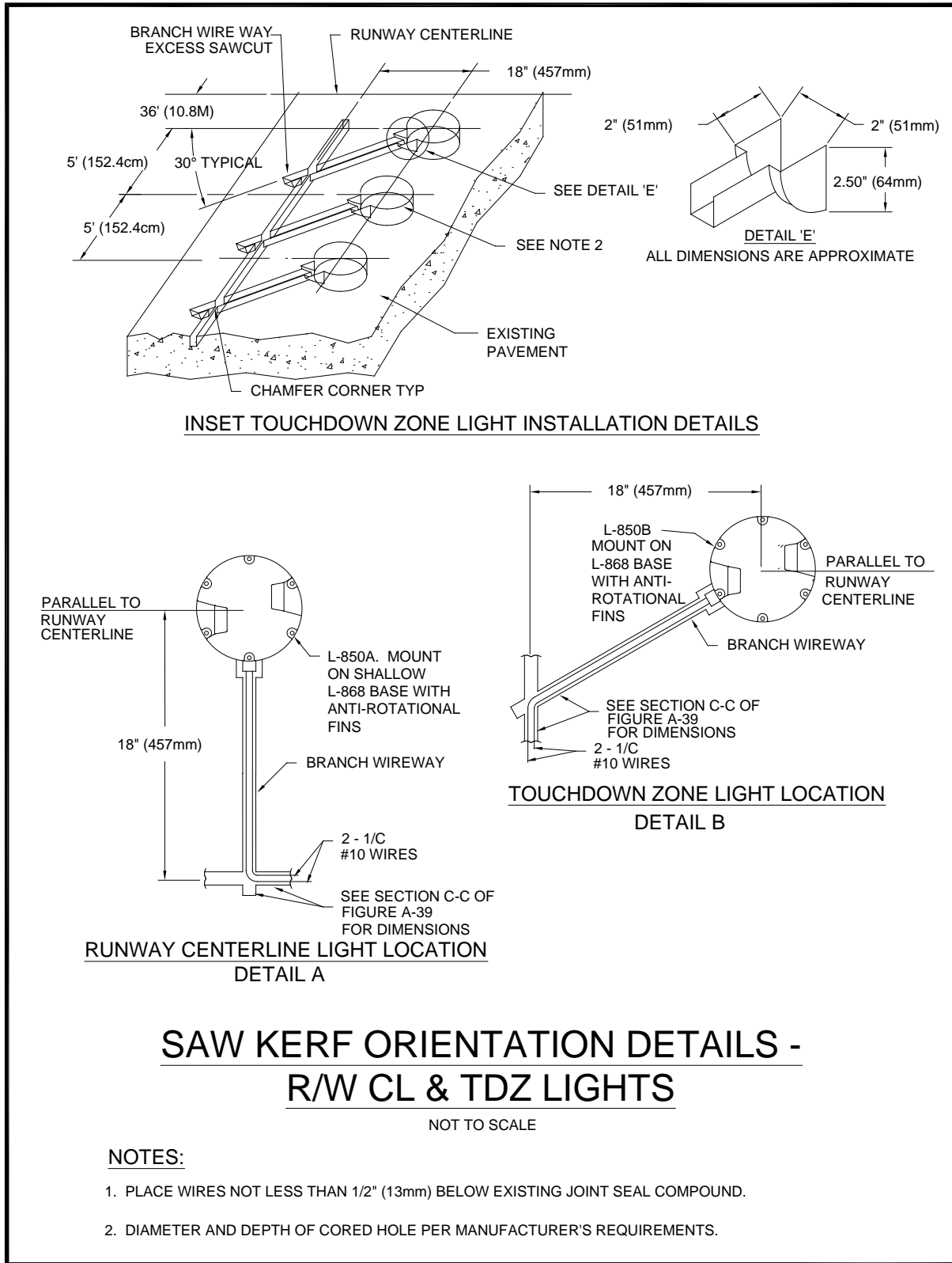
Figure A-40. Saw Kerf Orientation Details – R/W Centerline and Touchdown Zone (TDZ) Lights
