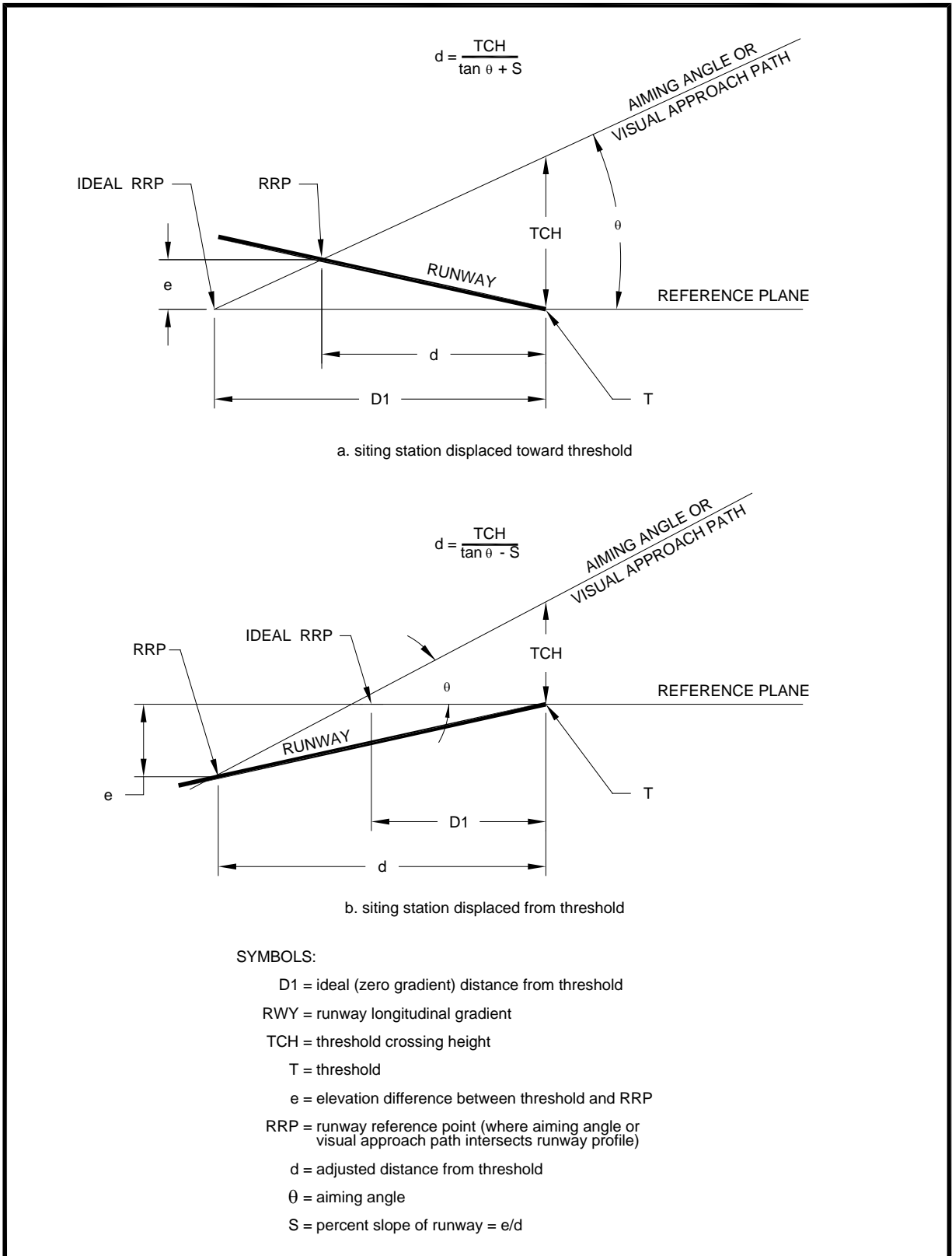
Figure A-83. Correction for Runway Longitudinal Gradient
