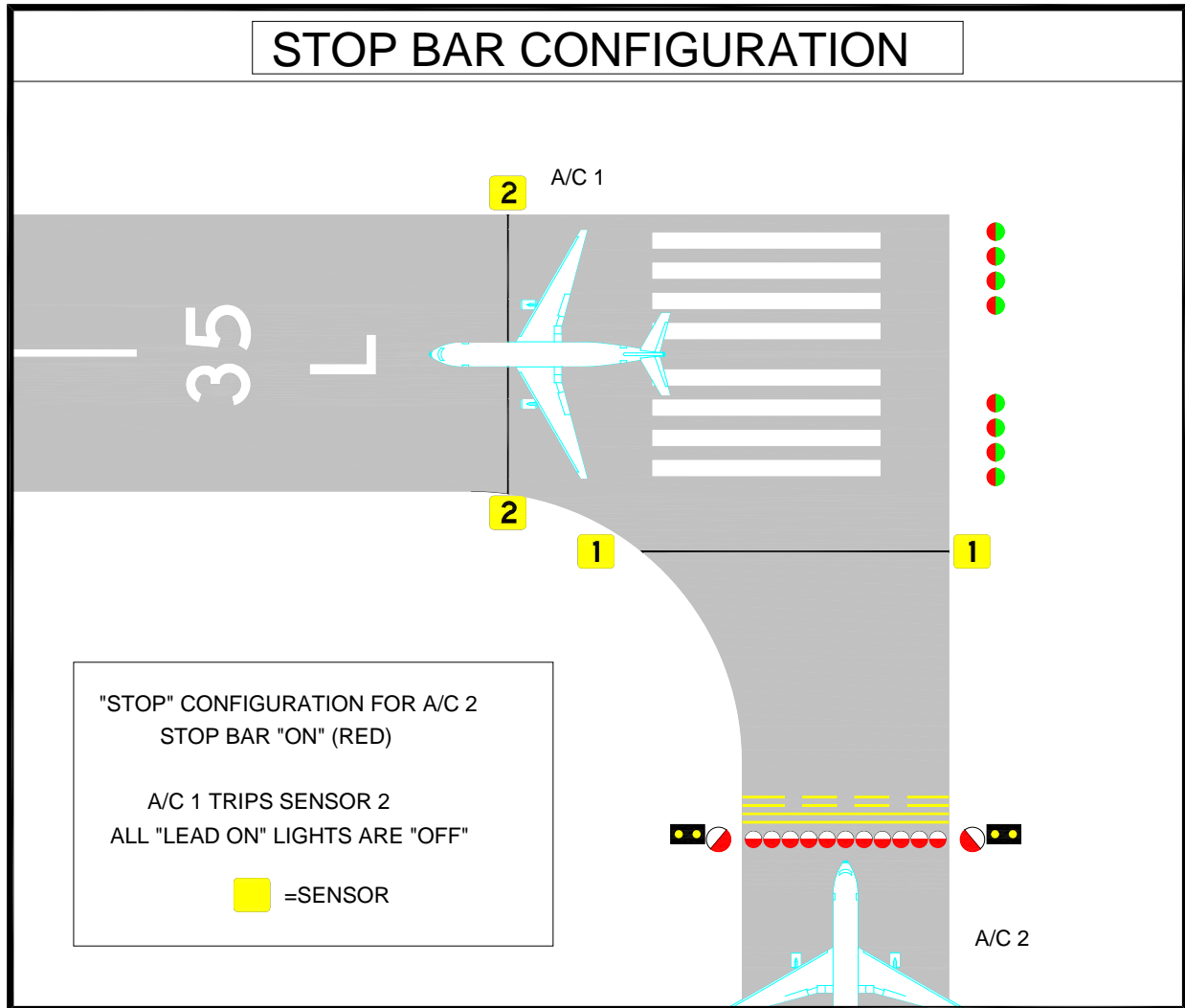
Figure A-62. Controlled Stop Bar Design and Operation – “STOP” Configuration for A/C 2
