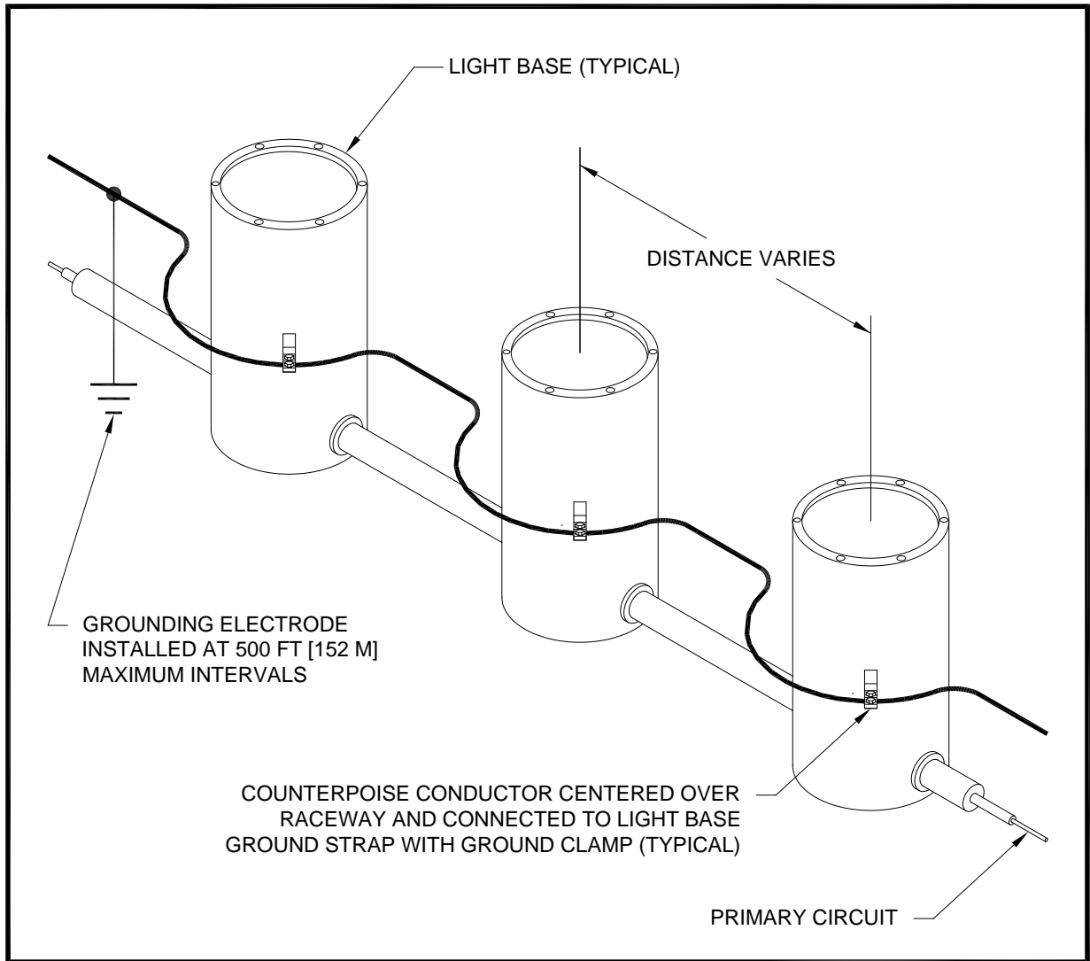
Figure A-111. Equipotential Counterpoise Installation Method
