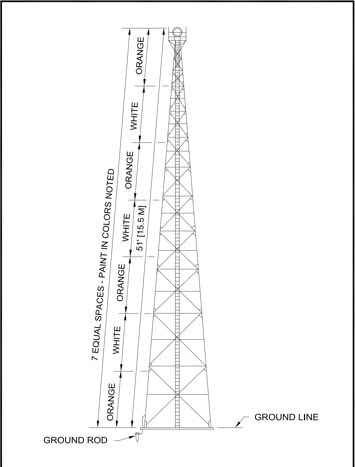
Figure A-72. Typical Structural Beacon Tower
