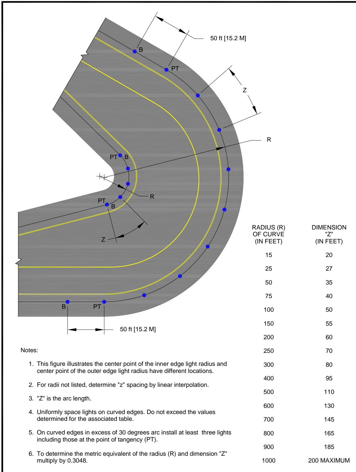
Figure A-16. Spacing of Lights on Curved Taxiway Edges
