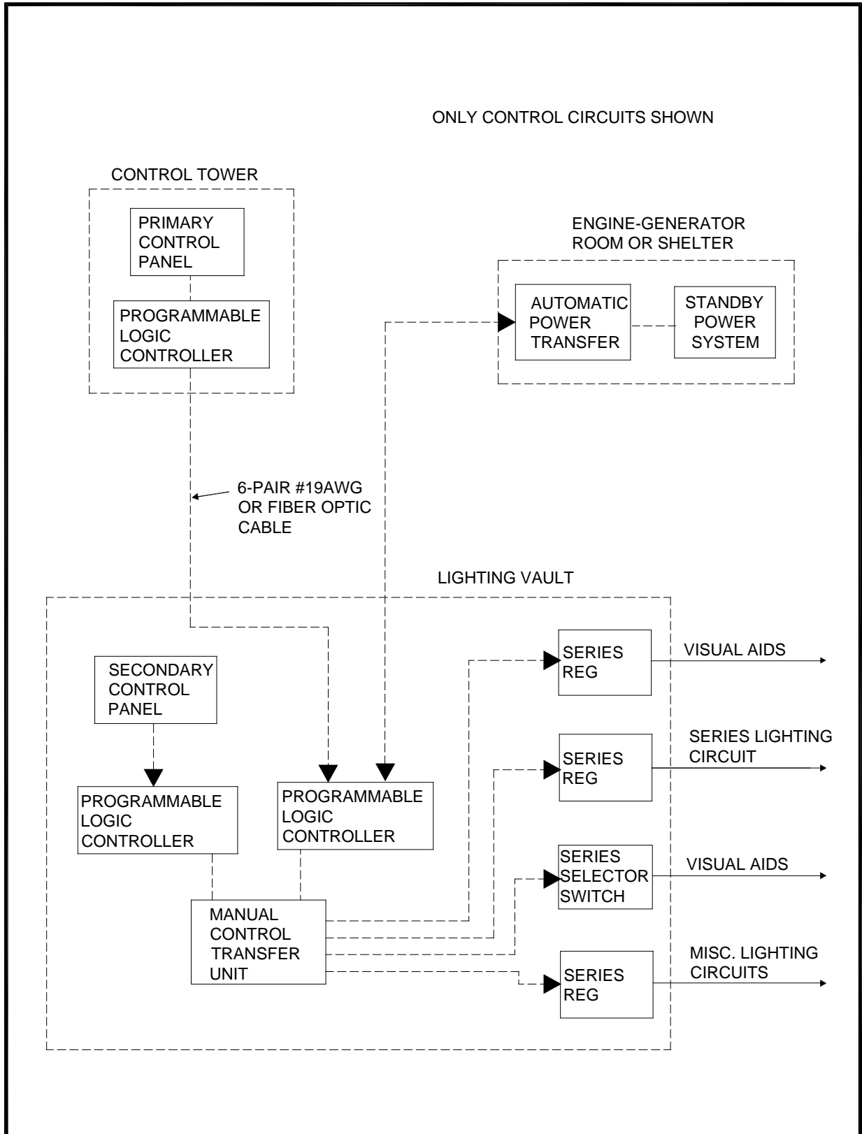
Figure A-114. Typical PLC Control System Block Diagram
