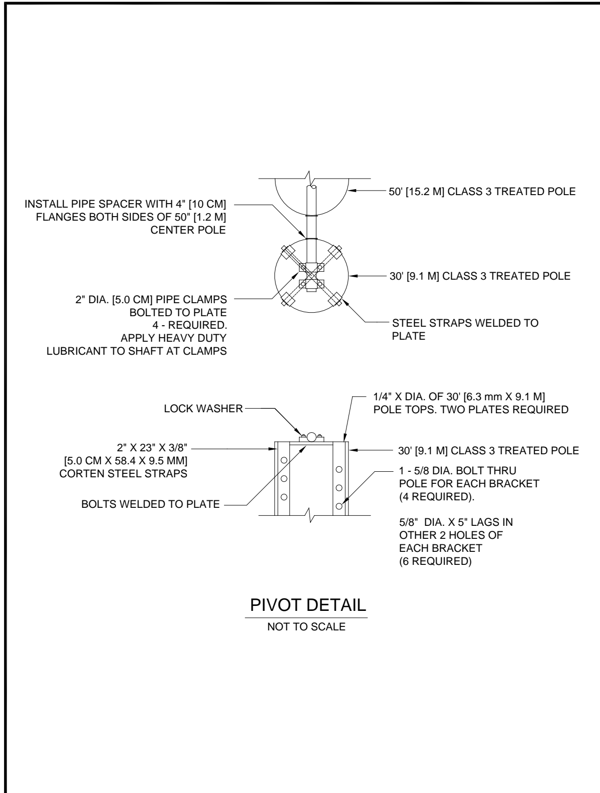
Figure E-17. Standard Details for Pivoting Rotating Beacon Pole – Pivot Detail
