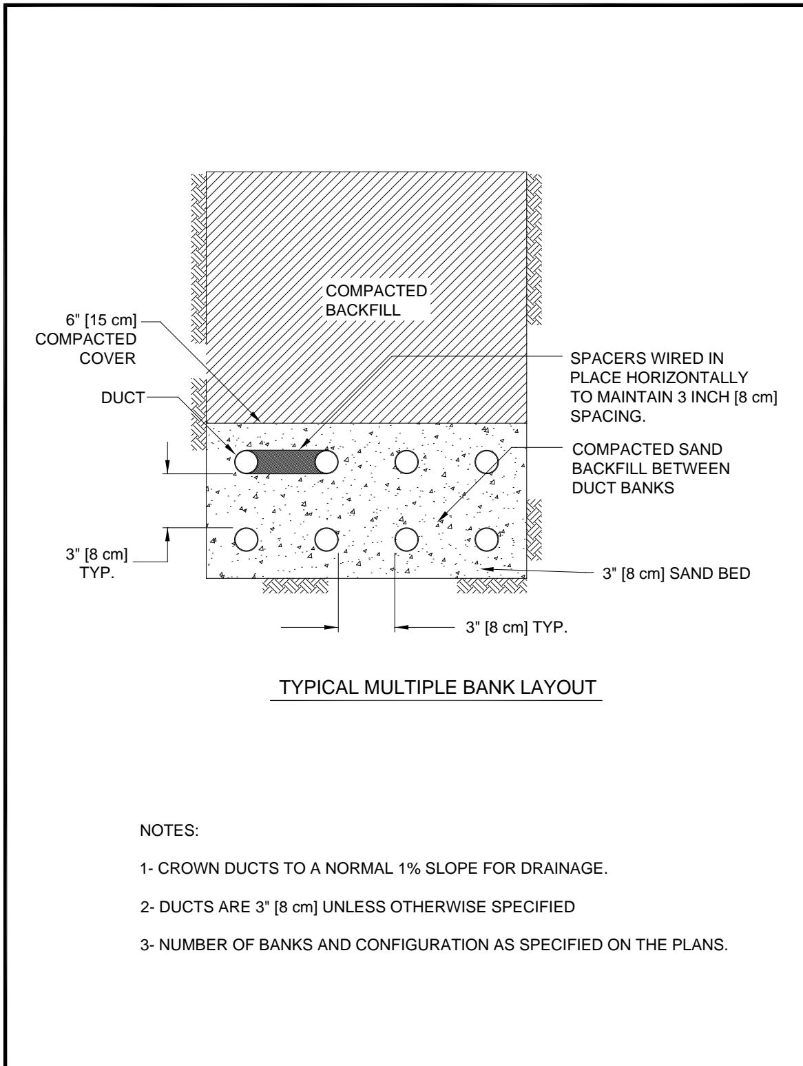
Figure E-6. Standard Details for Underground Cable Installation – Typical Multiple Bank Layout
