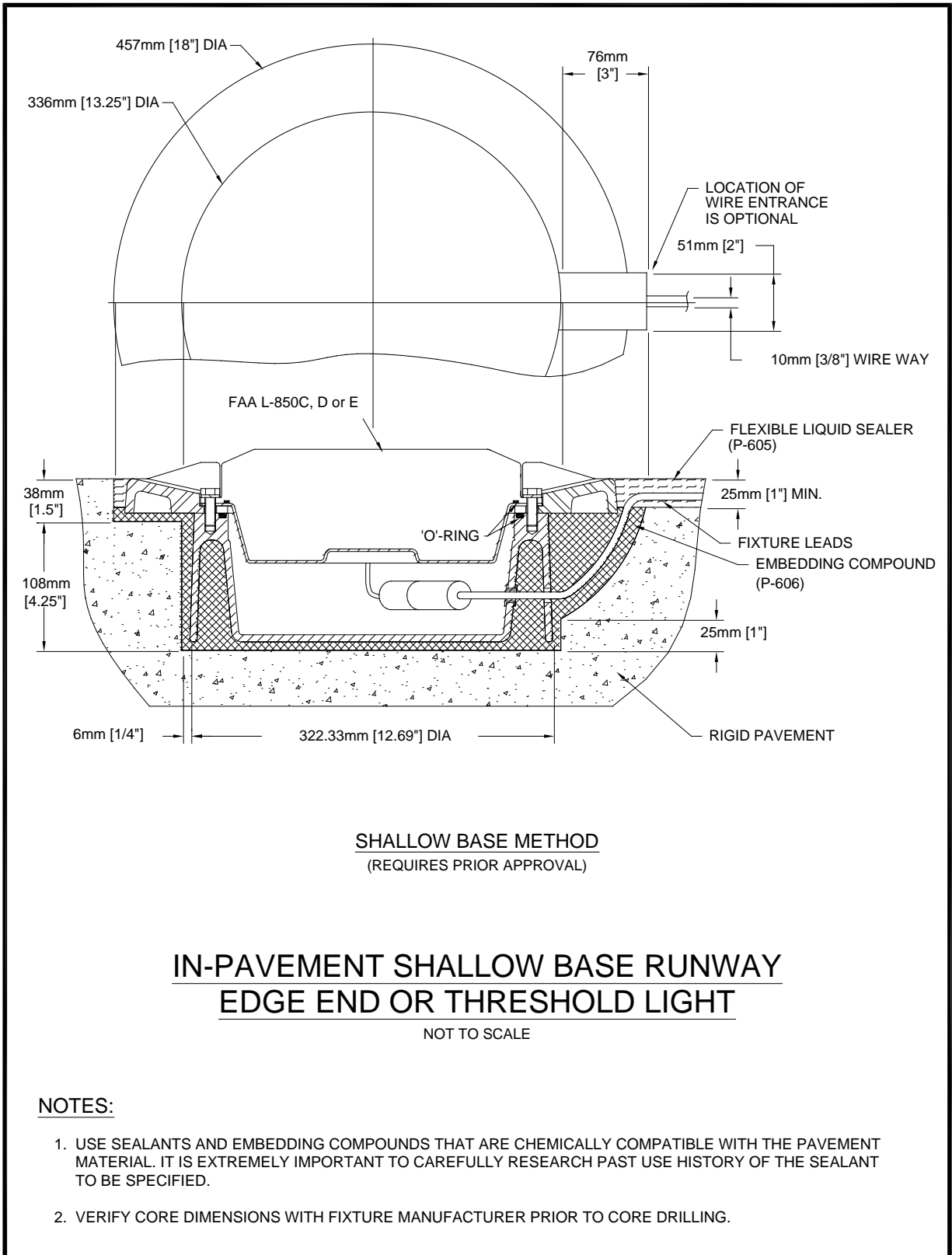
Figure A-104. In-pavement Shallow Base Runway Edge End or Threshold Light
