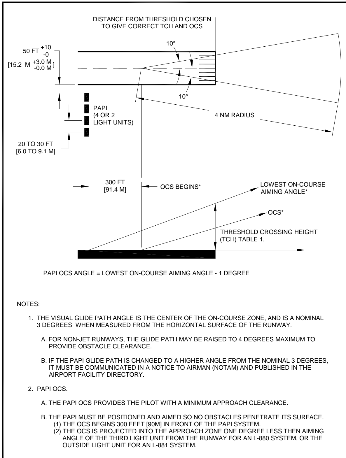
Figure A-81. PAPI Obstacle Clearance Surface
