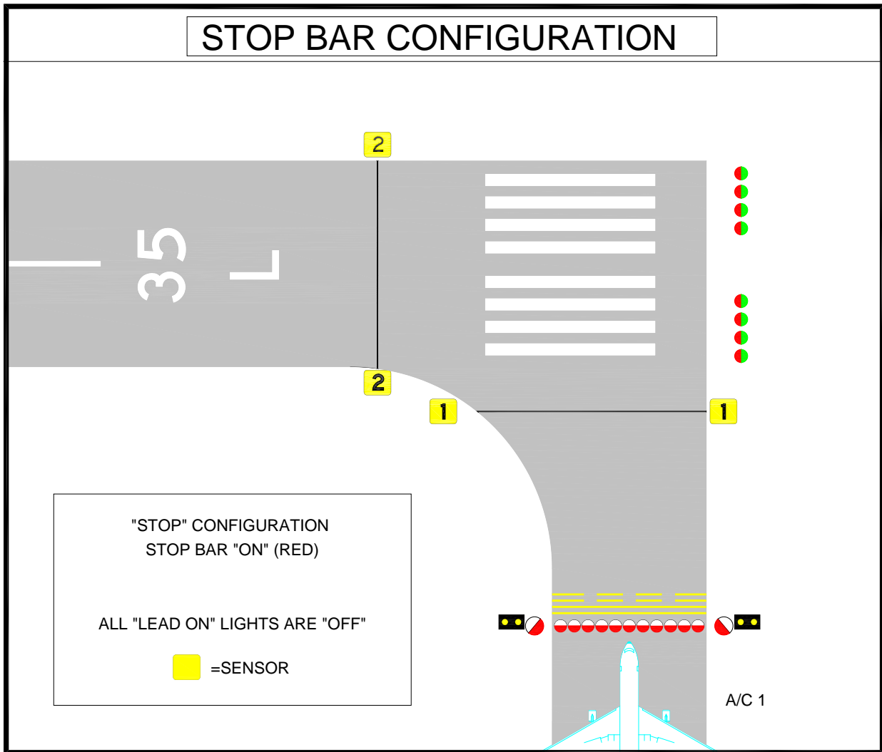
Figure A-60. Controlled Stop Bar Design and Operation – “STOP” Configuration
