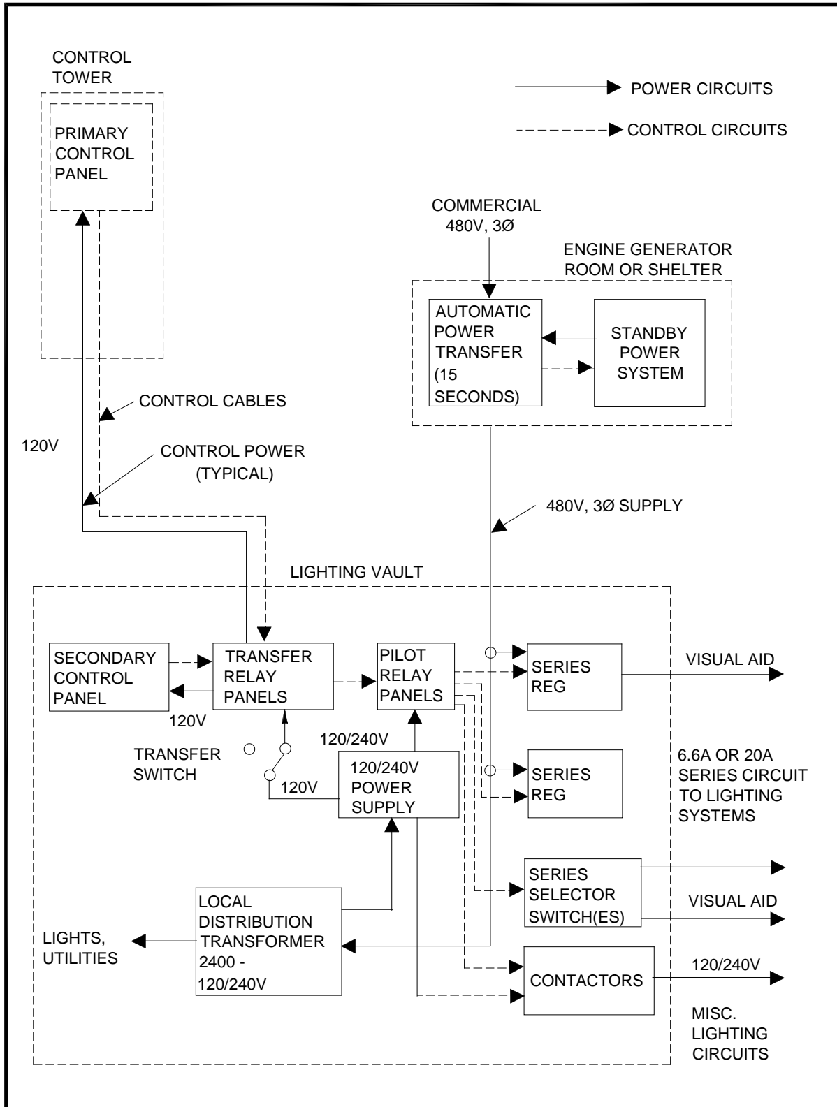
Figure A-113. Power and Control System Block Diagram
