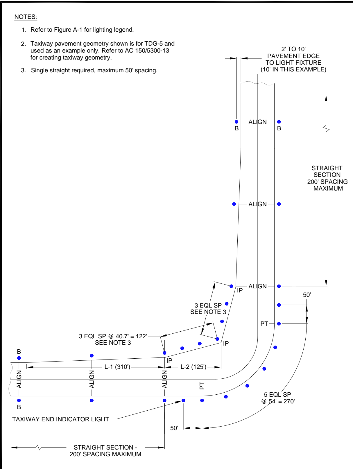
Figure A-17. Taxiway Edge Lights for Standard Taxiway Turns
