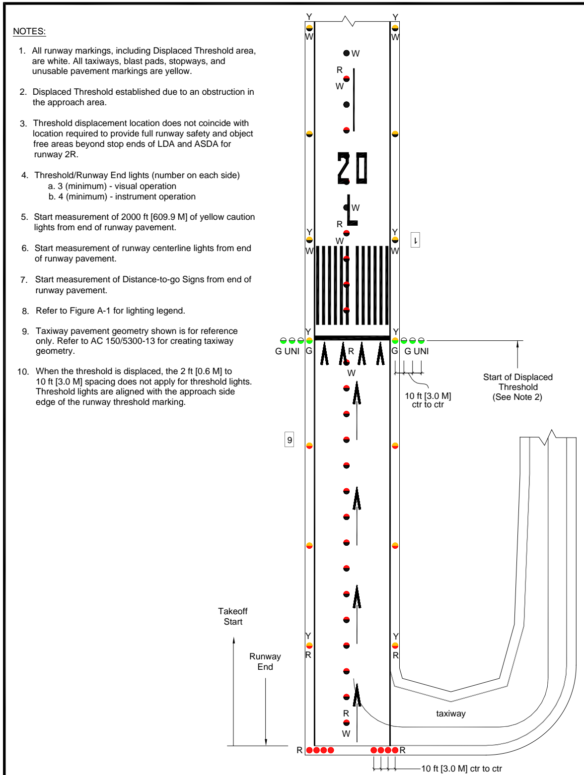
Figure A-9. Lighting for Runway with Displaced Threshold Not Coinciding with Opposite Runway End
