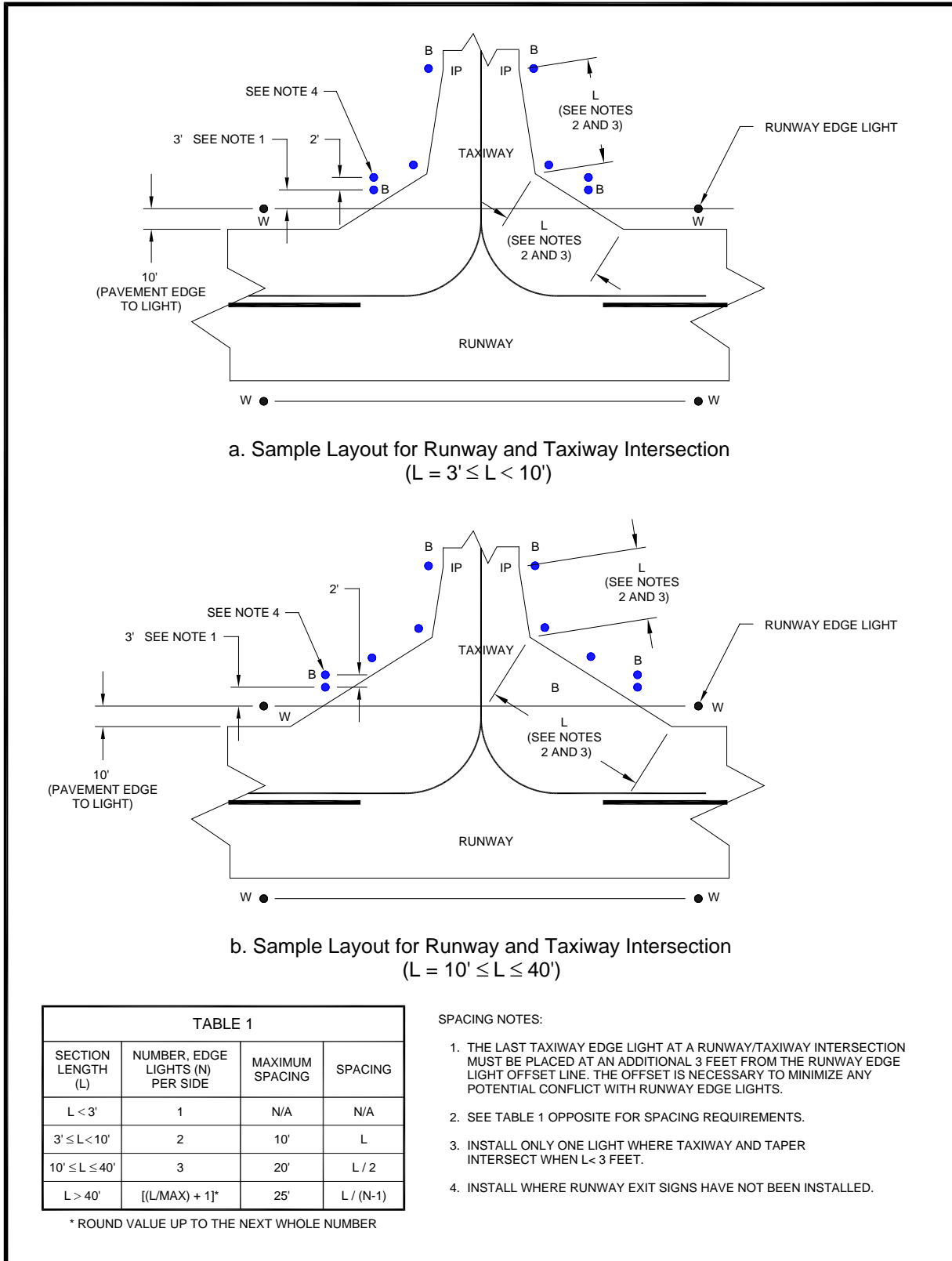
Figure A-18. Taxiway Edge Lights for Runway/Taxiway Intersection
