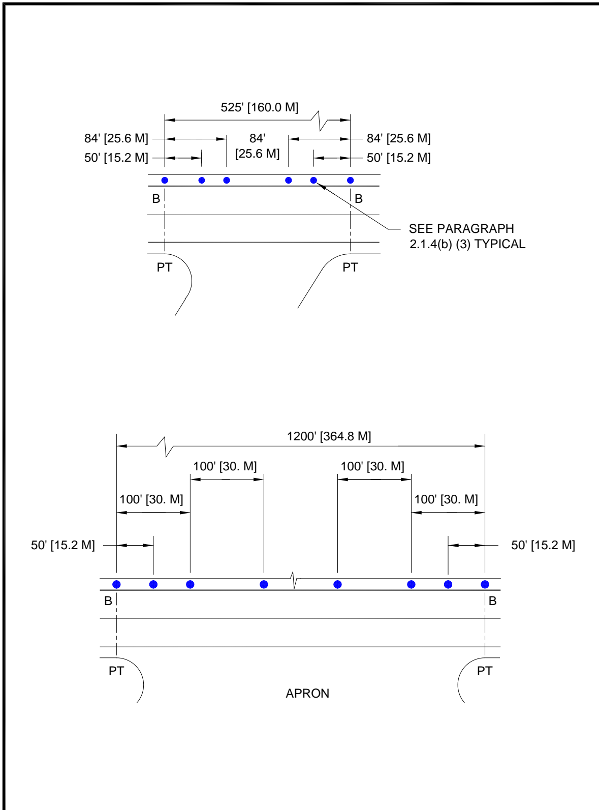
Figure H-13. Typical Single Straight Taxiway Edges (More Than 200 ft (61 m)) (Legacy Figure 18)
