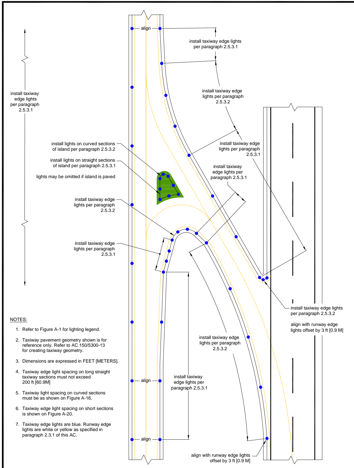
Figure A-21. Lighting for Typical High-Speed Exit Taxiway
