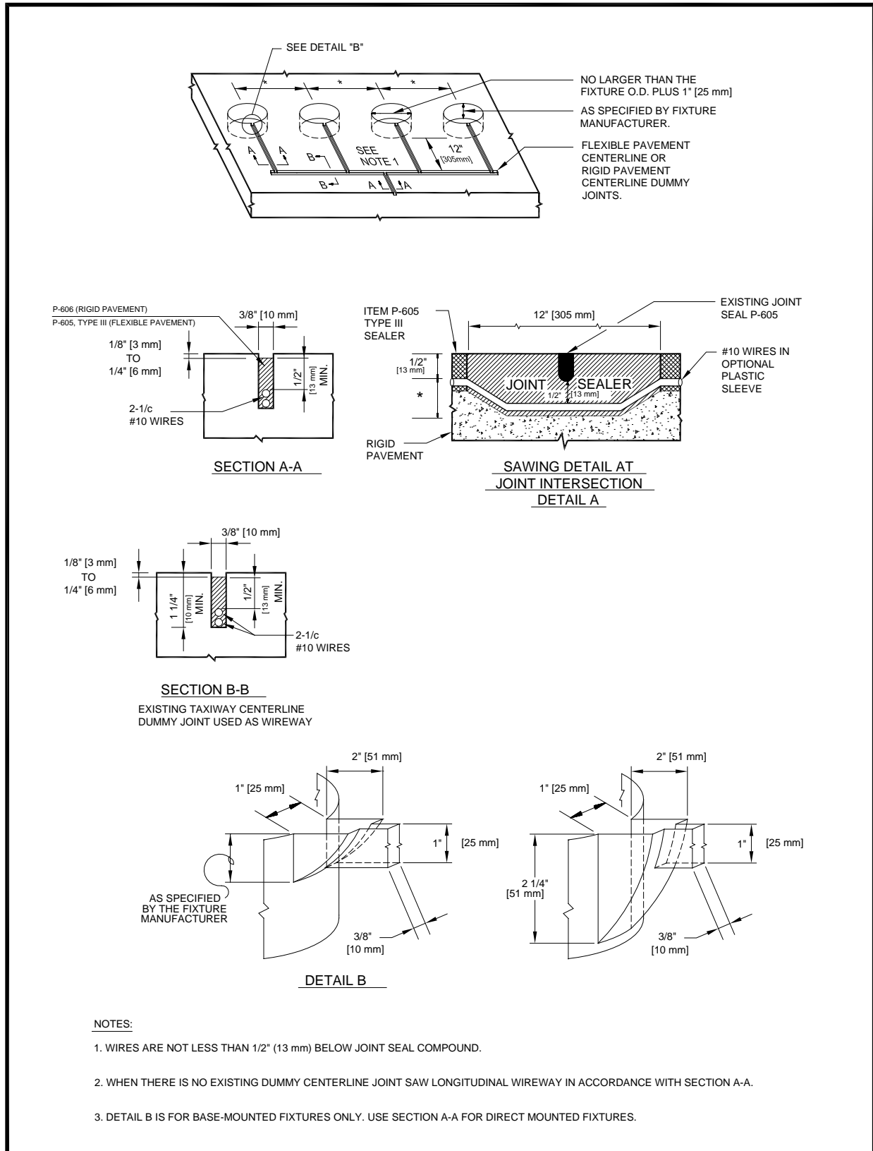
Figure A-106. Sawing and Drilling Details for In-Pavement Taxiway Centerline Lights
