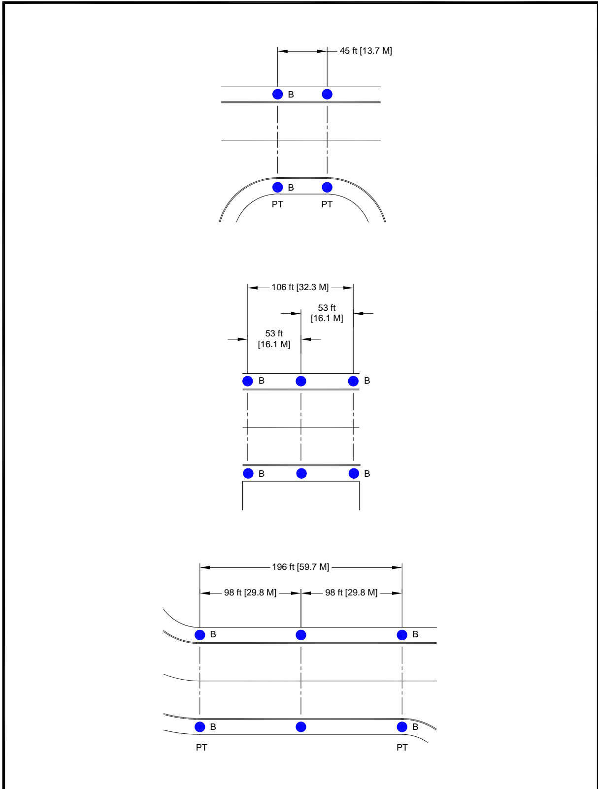
Figure H-11. Typical Straight Taxiway Sections (Less Than 200 ft (61 m)) (Legacy Figure 16)
