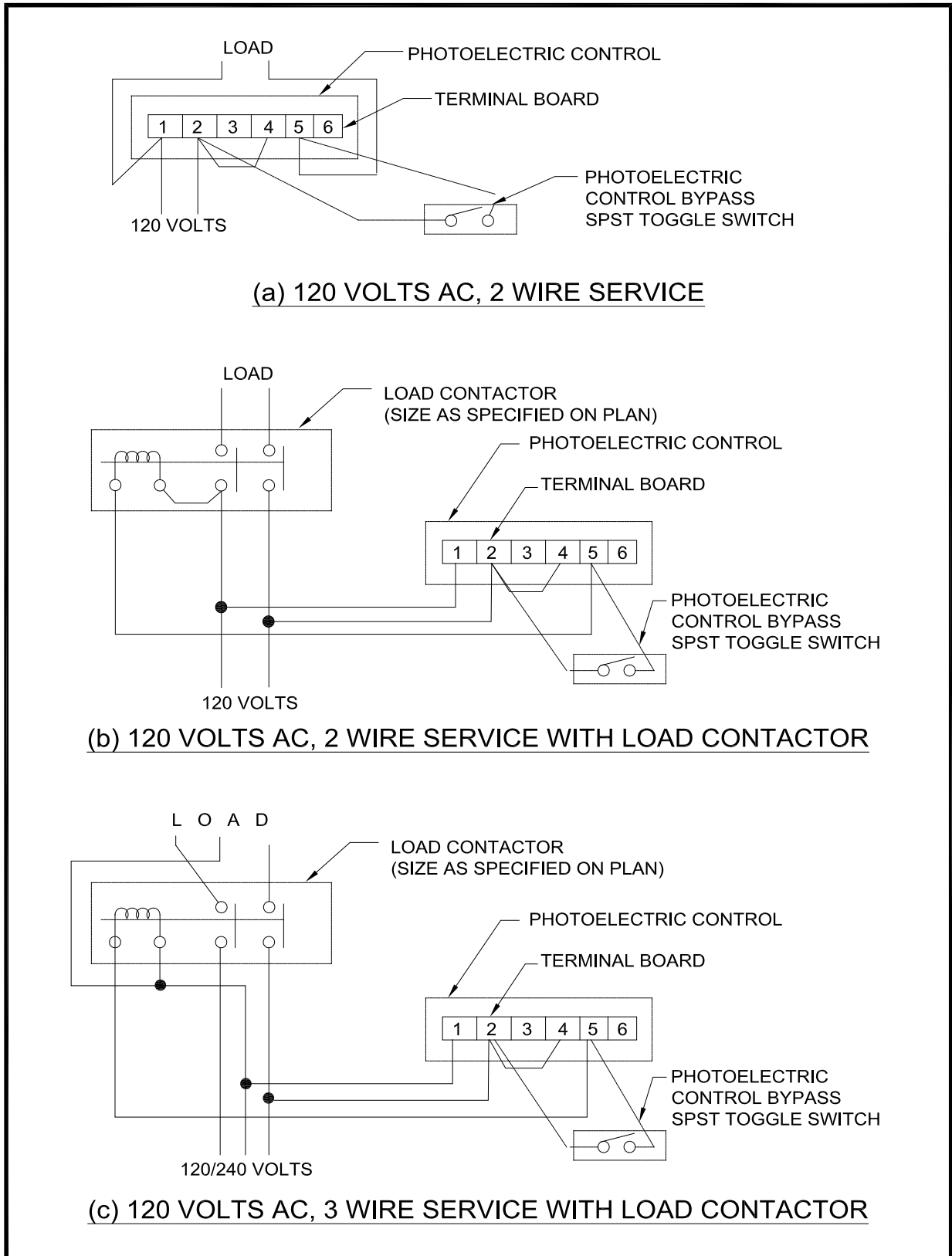
Figure A-70. Typical Automatic Control
