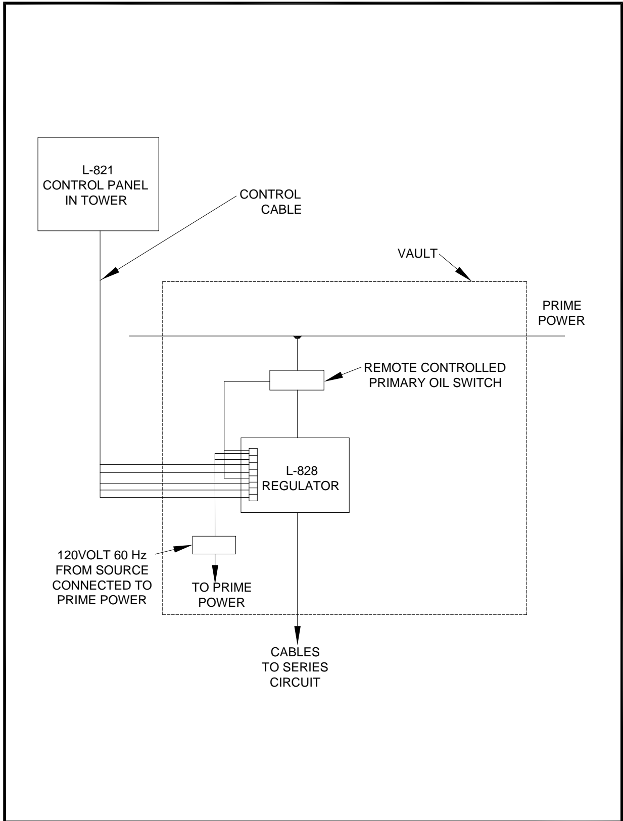
Figure A-100. Typical Wiring Diagram for Configuration “C” Power
