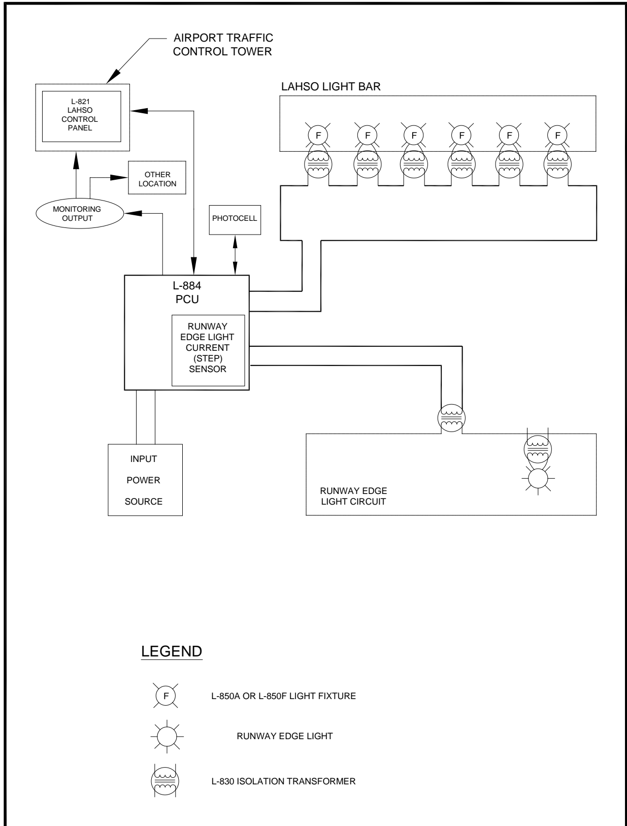
Figure A-66. Typical Block Diagram for Land and Hold Short Lighting System
