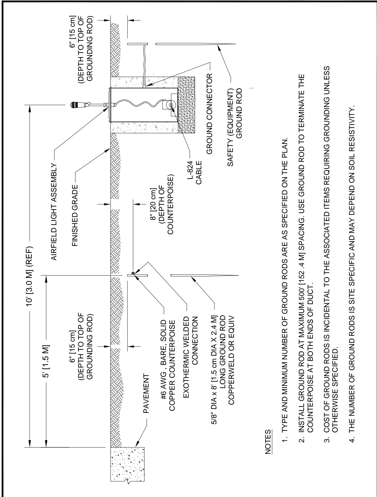
Figure A-112. Isolation Counterpoise Installation Method
