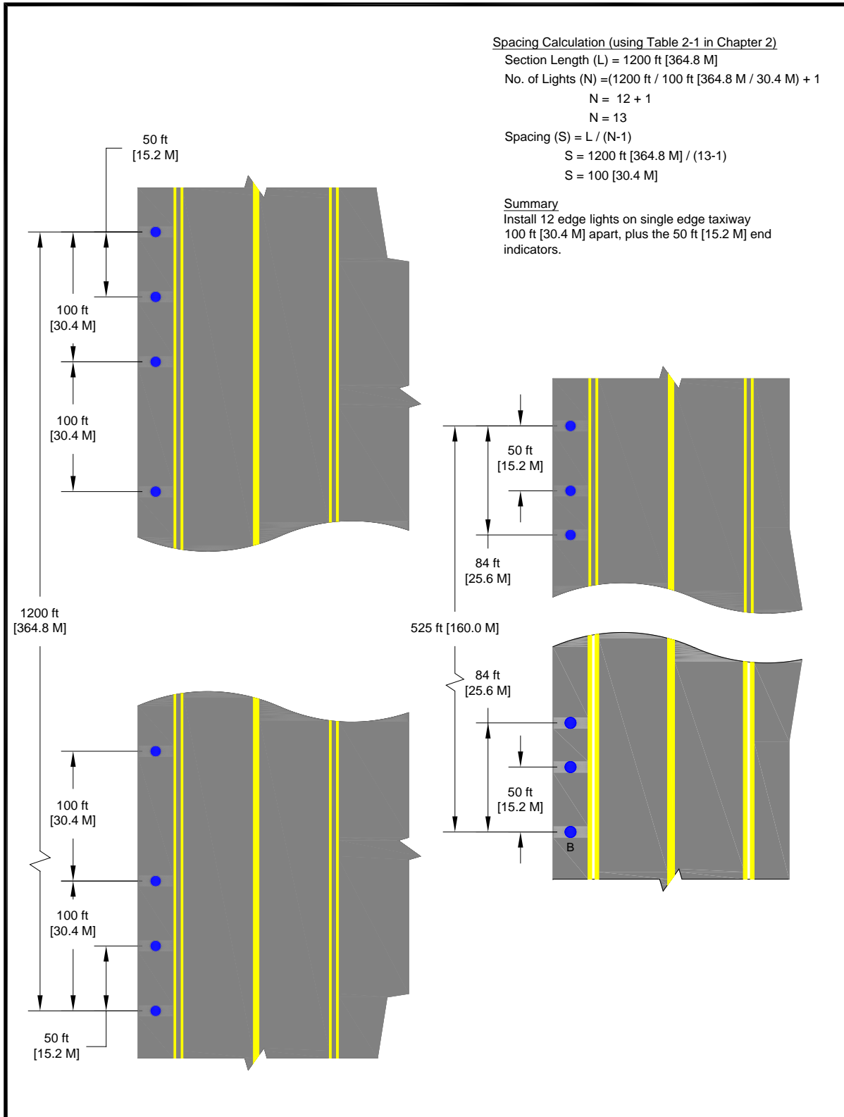
Figure A-19. Typical Single Straight Taxiway Edges (200 feet or More (61 m))
