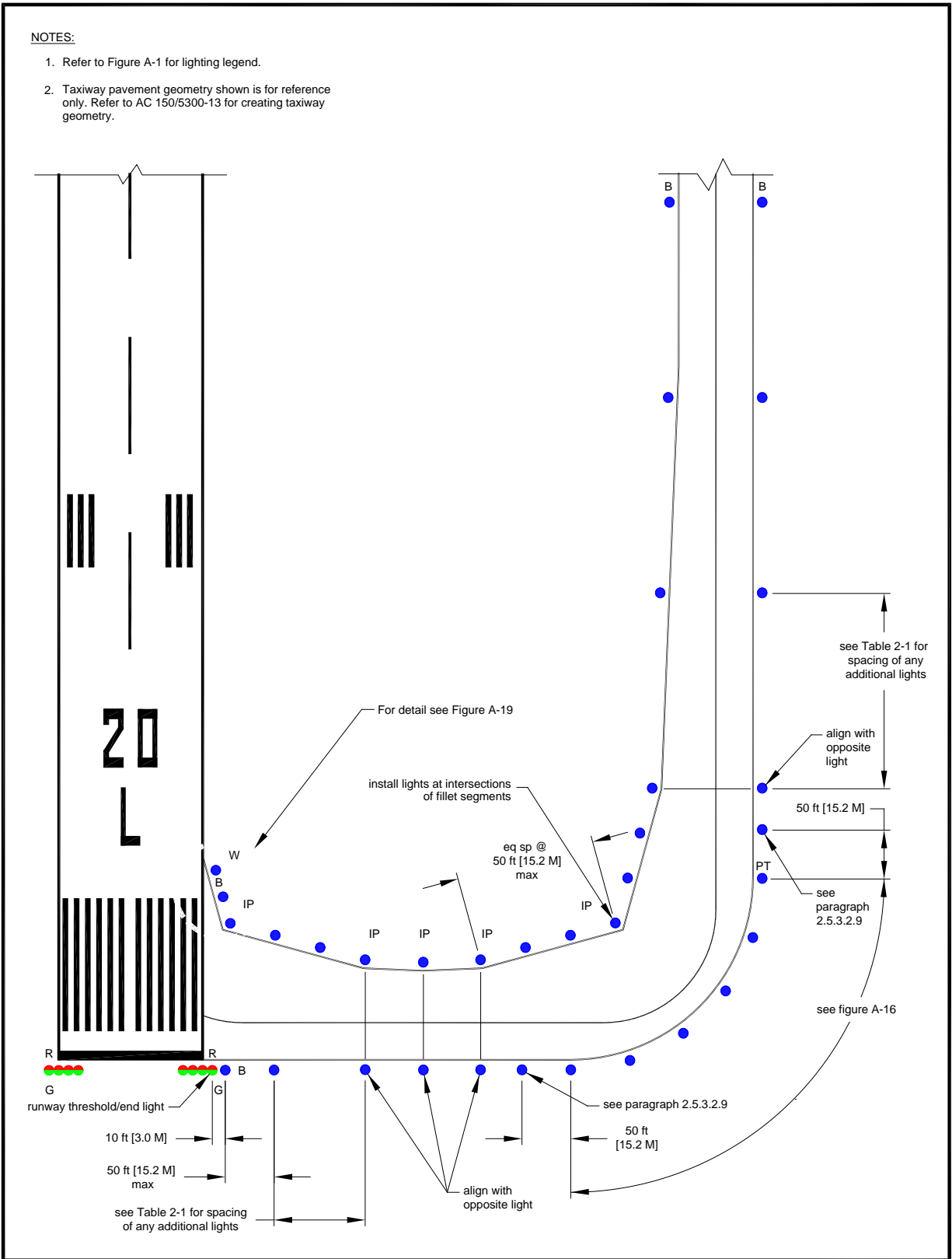
Figure A-13. Lighting for Typical Runway Entrance
