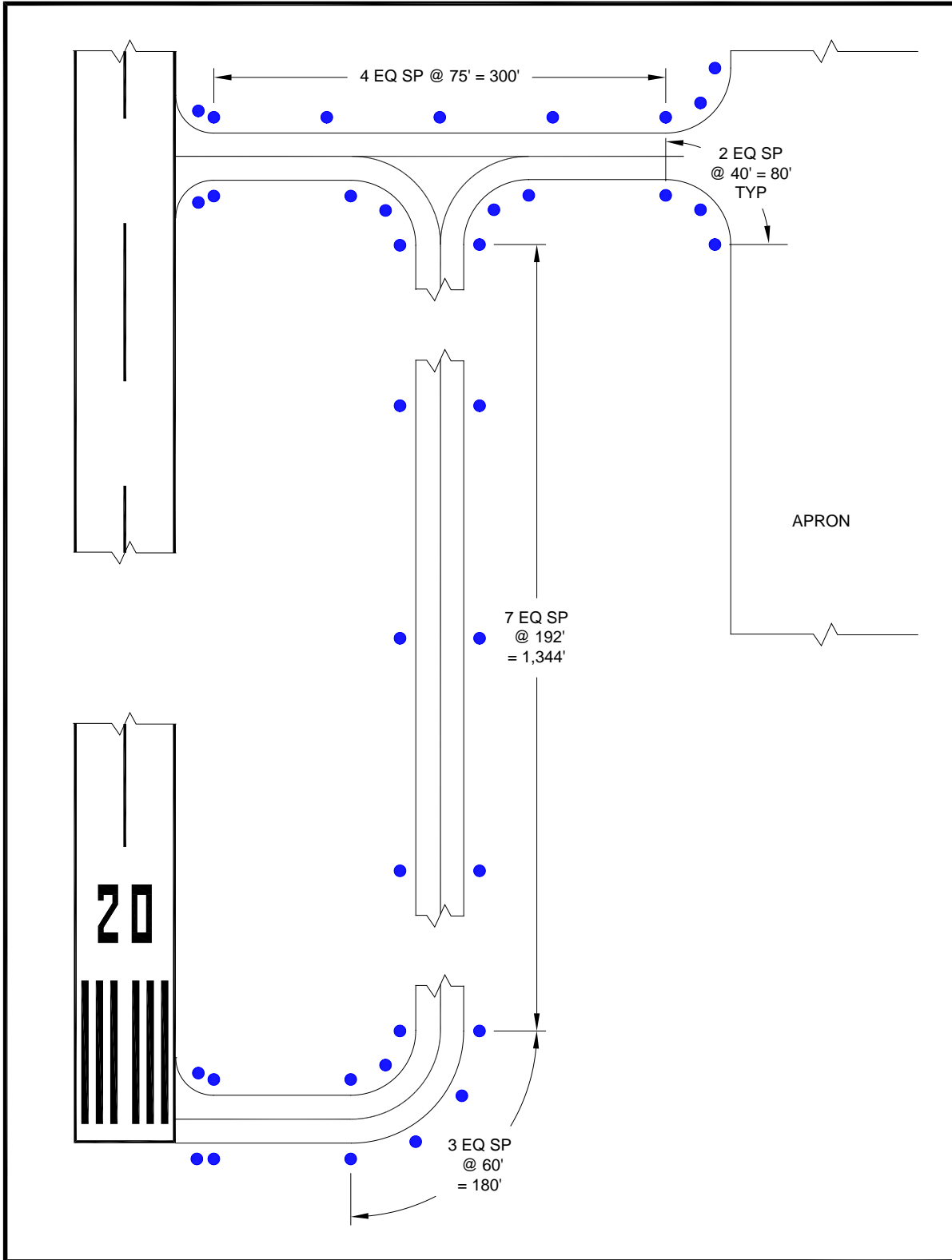
Figure A-116. Typical Spacing for GA Airport Edge Lights
