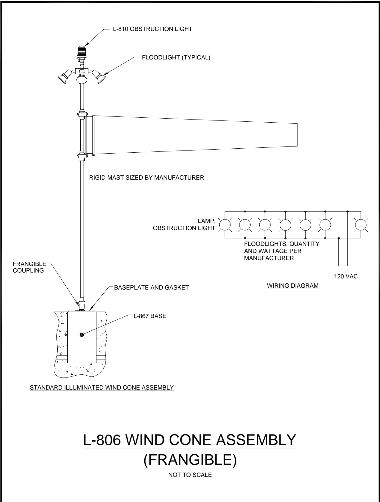
Figure A-77. Externally Lighted Wind Cone Assembly (Frangible)
