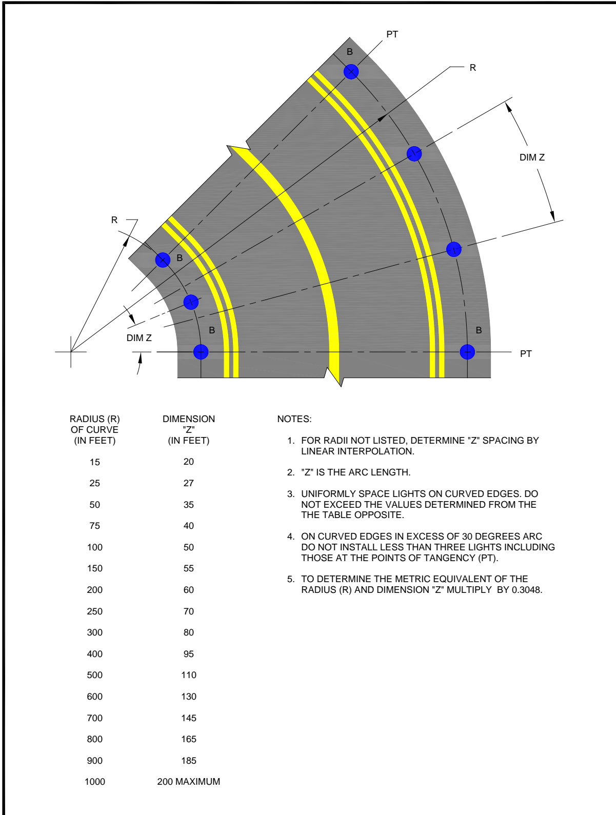
Figure H-12. Spacing of Lights on Curved Taxiway Edges (Legacy Figure 17)
