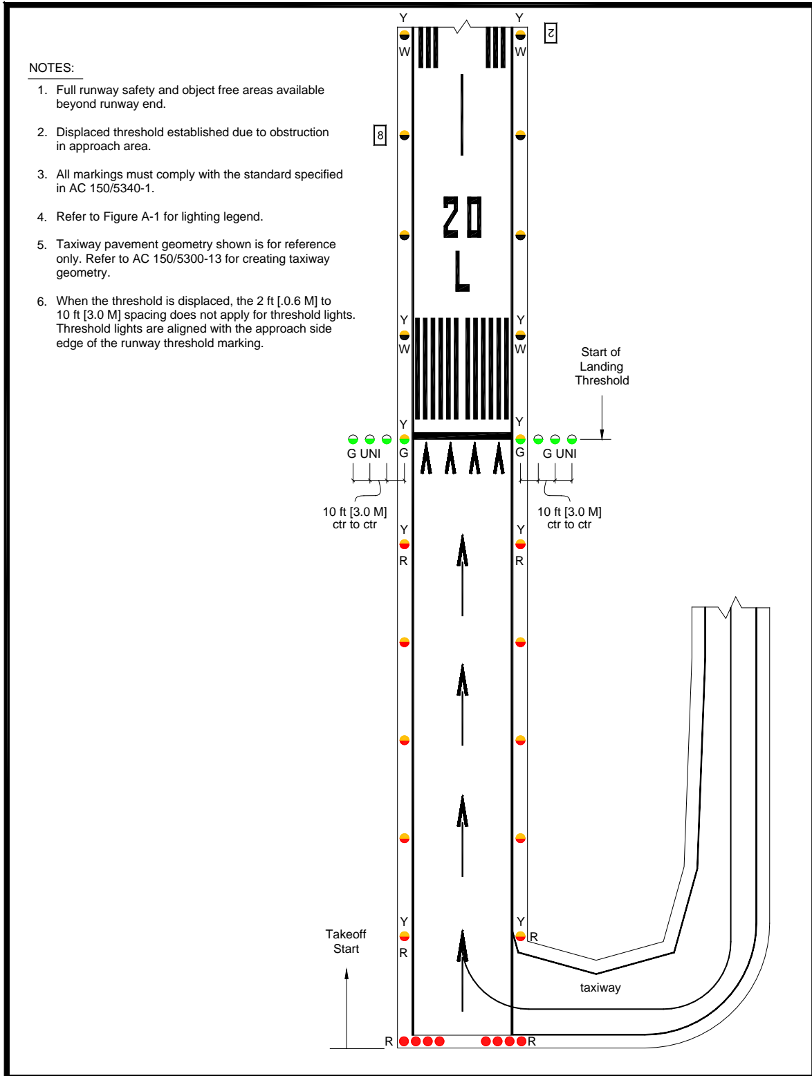
Figure A-5. Lighting for Runway with Displaced Threshold
