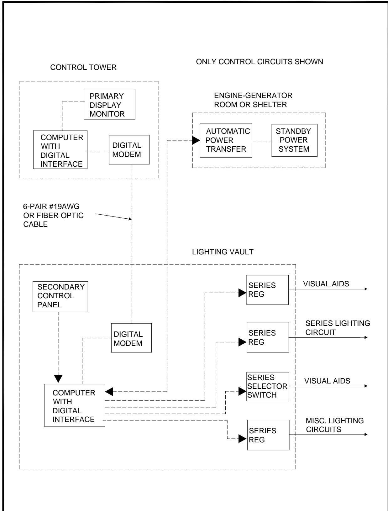
Figure A-115. PC Control System Block Diagram
