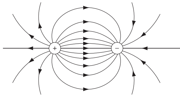
Opposite charges
