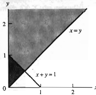
Figure 4.1.1. Regions for Example 4.1.12
