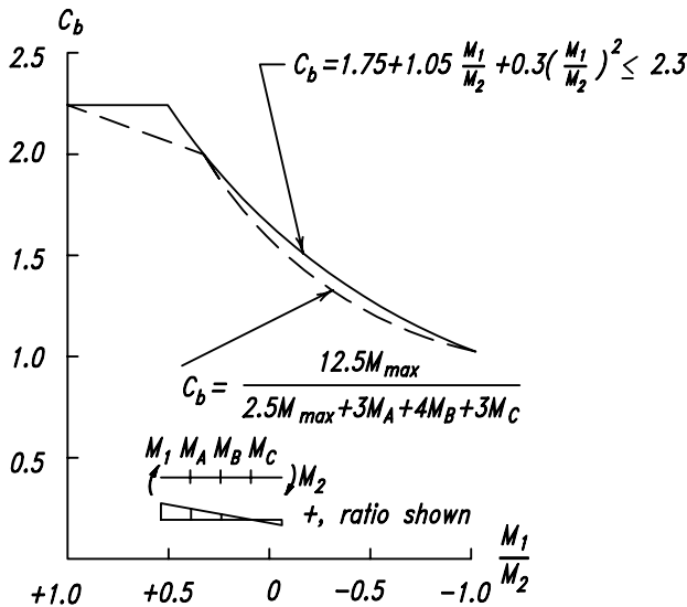
C-F1.3. C_b for a straight line moment diagram—prismatic beam.
