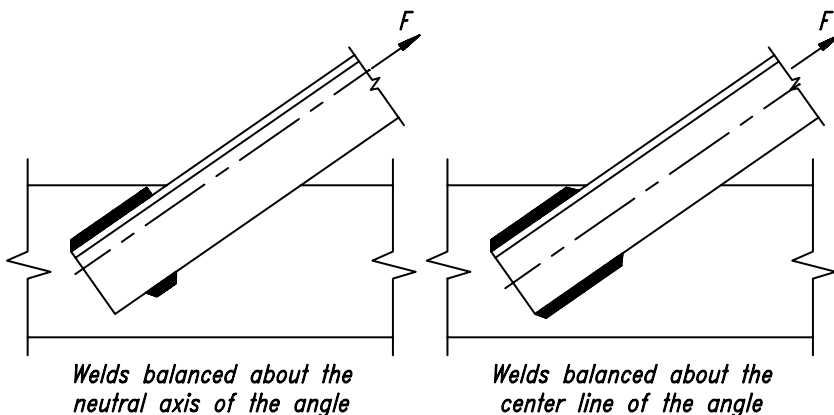
Figure C-J1.3. Balanced welds.
