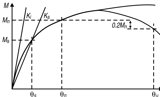
Fig. C-A2.1. Typical moment-rotation response of a partially-restrained connection.
