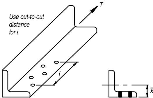
Fig. C-B3.2. Staggered holes.
