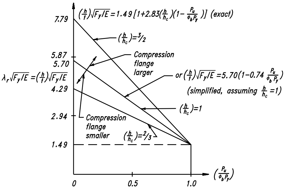
Fig. C-A-B5.1. Web local buckling for I-shaped members.
