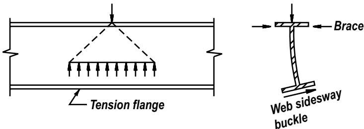
Fig. C-K1.1. Web sidesway buckling.
