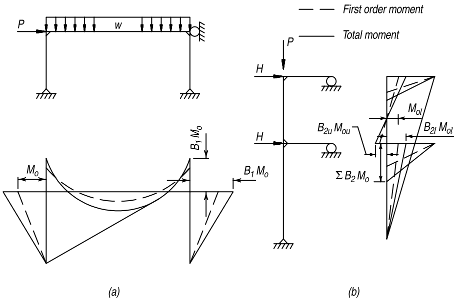
Fig. C-C1.1. Moment amplification.
