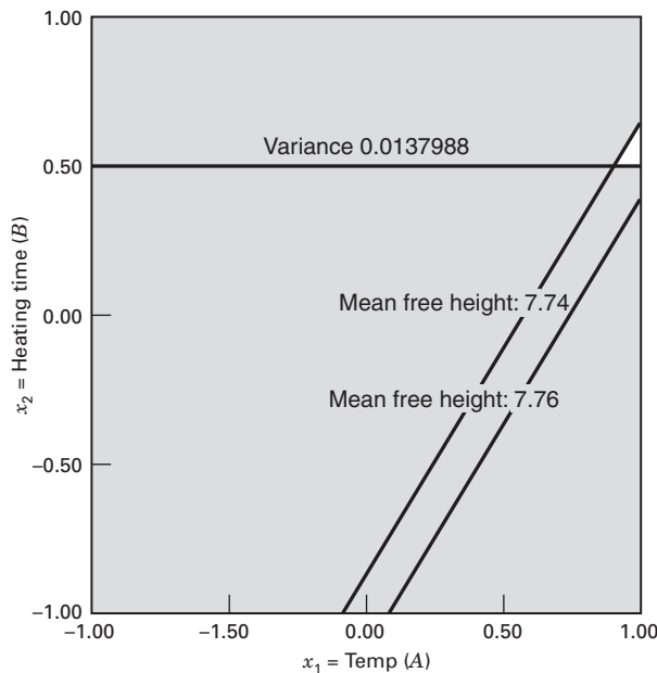
■ FIGURE 12.6 Overlay plot of the mean free height and variance of free height with x_4 = \text{hold down time } (D) \text{ at the high level}
