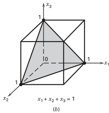
■ FIGURE 11.39 Constrained factor space for mixtures with (a) p = 2 components and (b) p = 3 components
