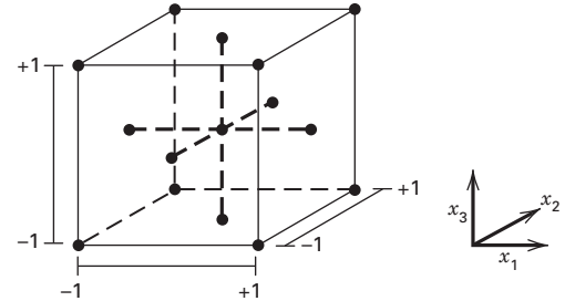
■ FIGURE 11.23 A face-centered central composite design for k = 3
