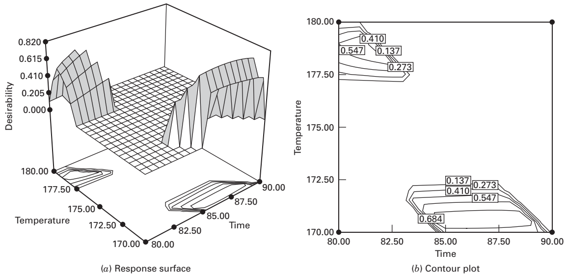
■ FIGURE 11.18 Desirability function response surface and contour plot for the problem in Example 11.2
