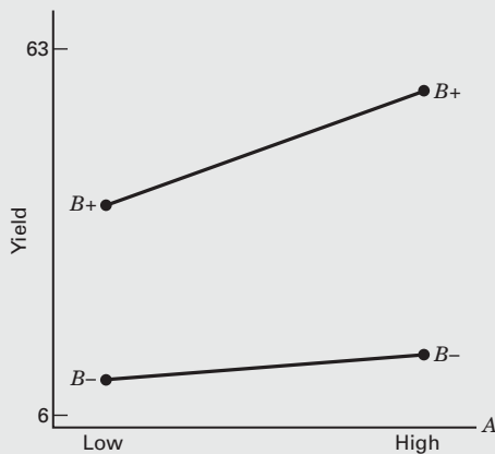
■ FIGURE 8.9 Aperture-exposure time interaction for Example 8.2
