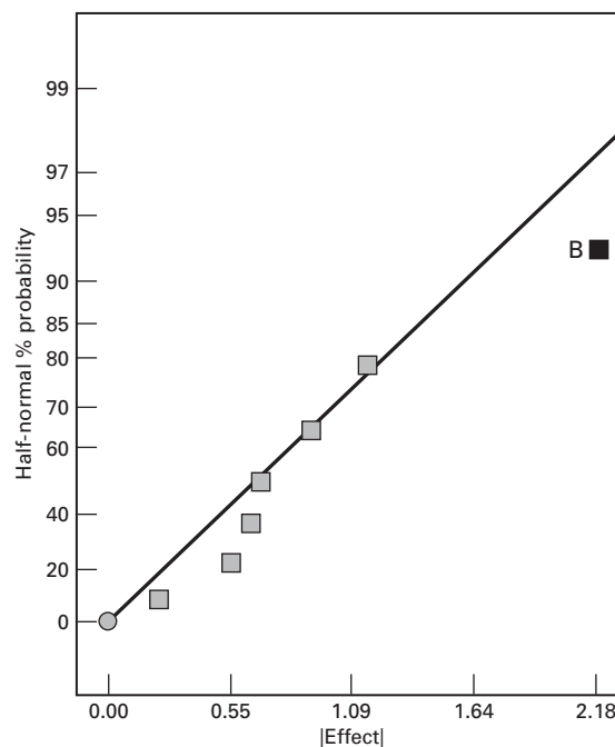
■ FIGURE 12.3 Half-normal plot of effects, \ln(s_i^2) response
